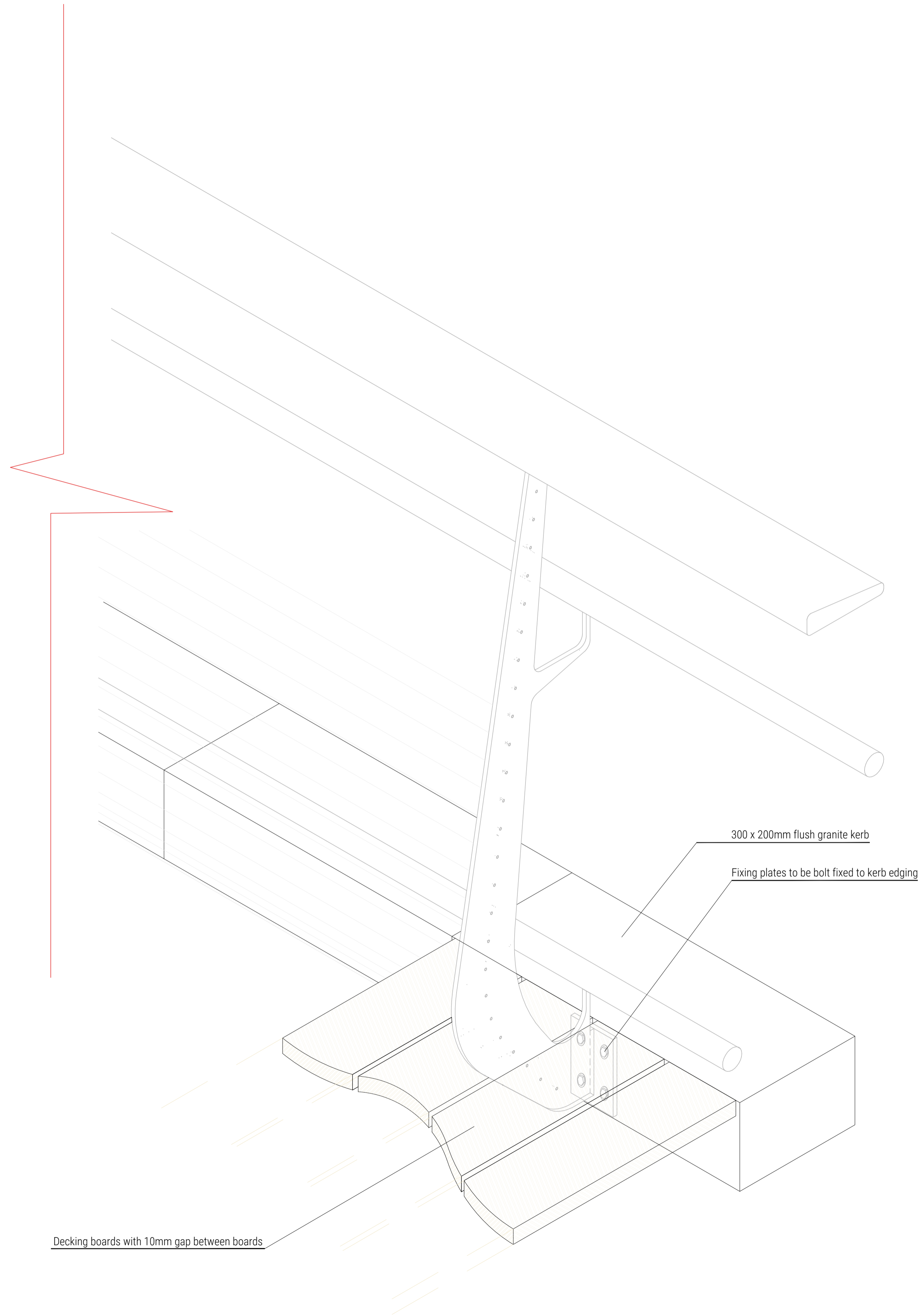
02 Handrail Type A Connection 02: Jetty L704 Isometric
