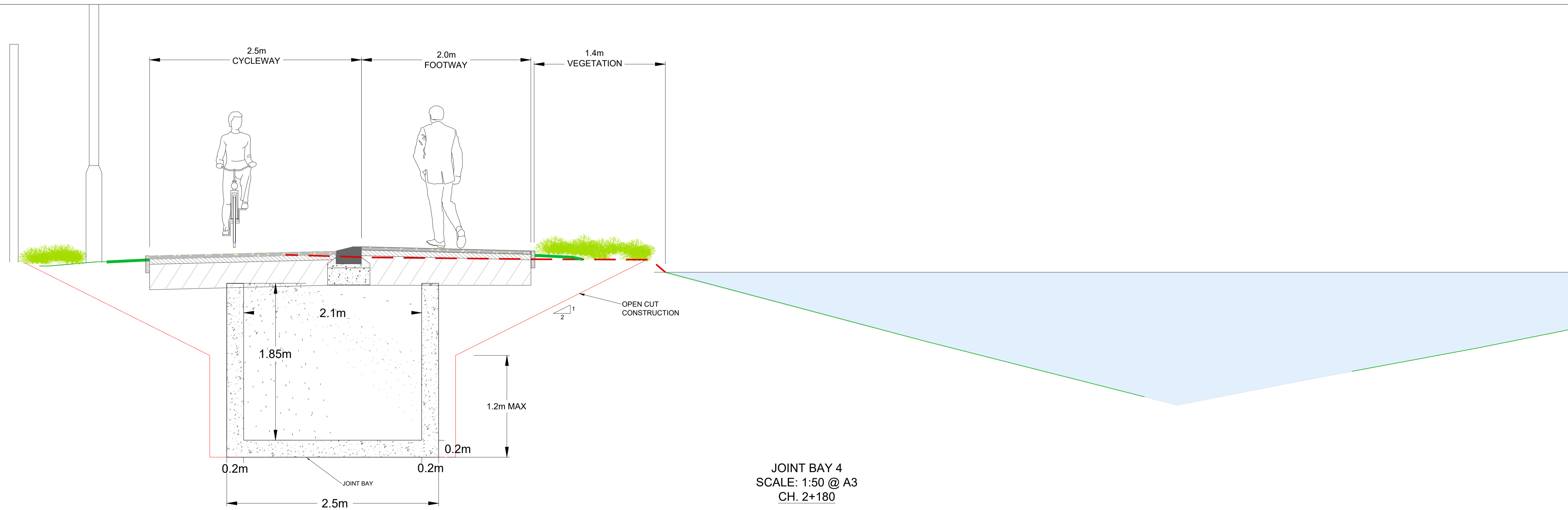
JOINT BAY 3 SCALE: 1:50 @ A3 LOCK 7 CH. 2+740
