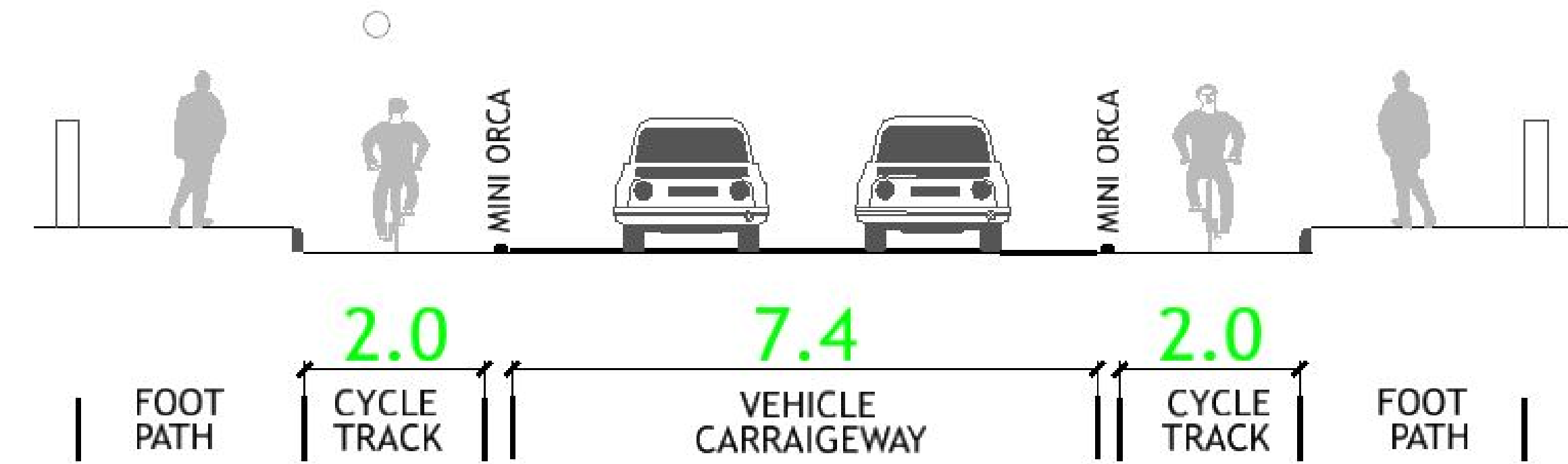
TYPICAL SECTION DETAIL
