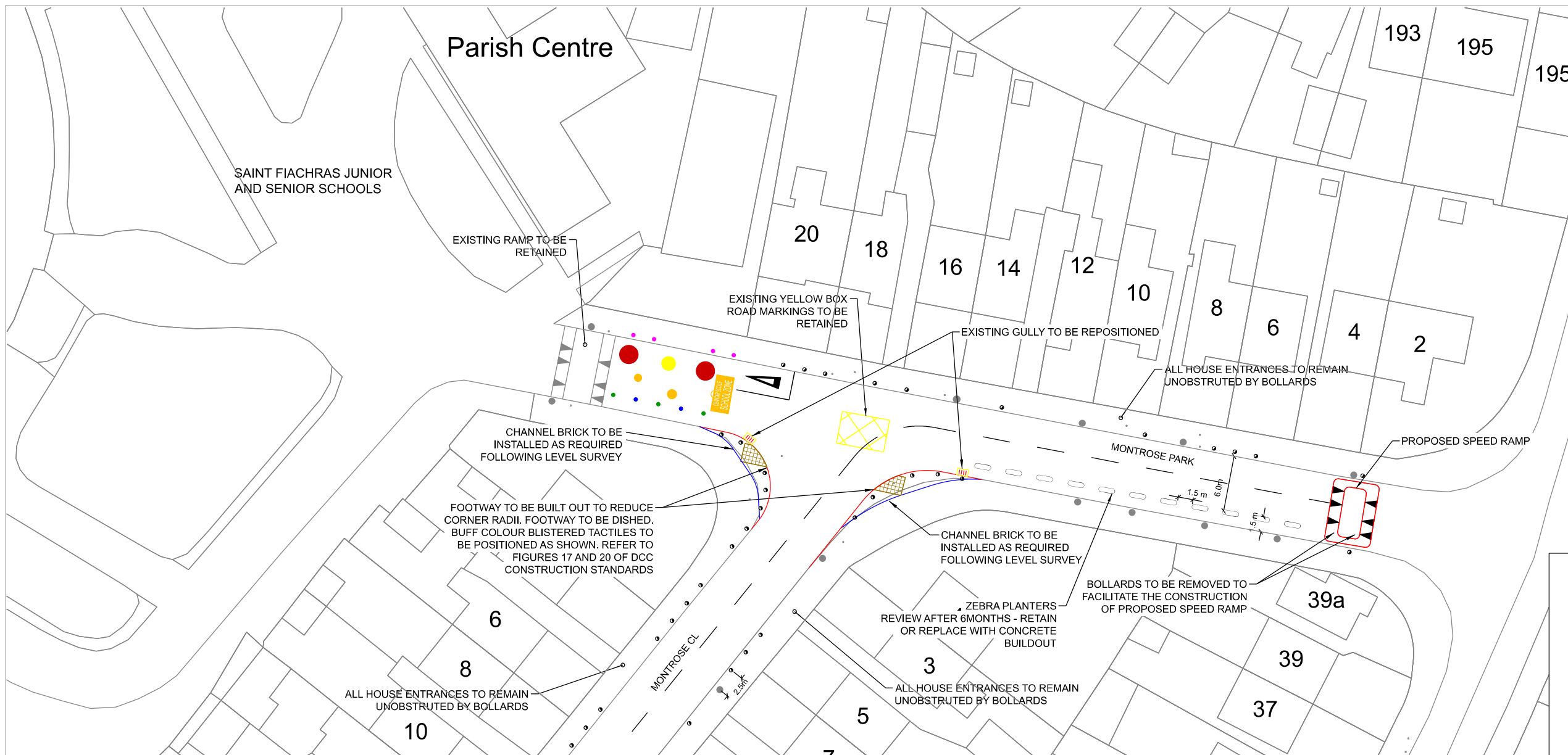
EXAMPLE OF ESTABLISHED ZEBRA PLANTERS
