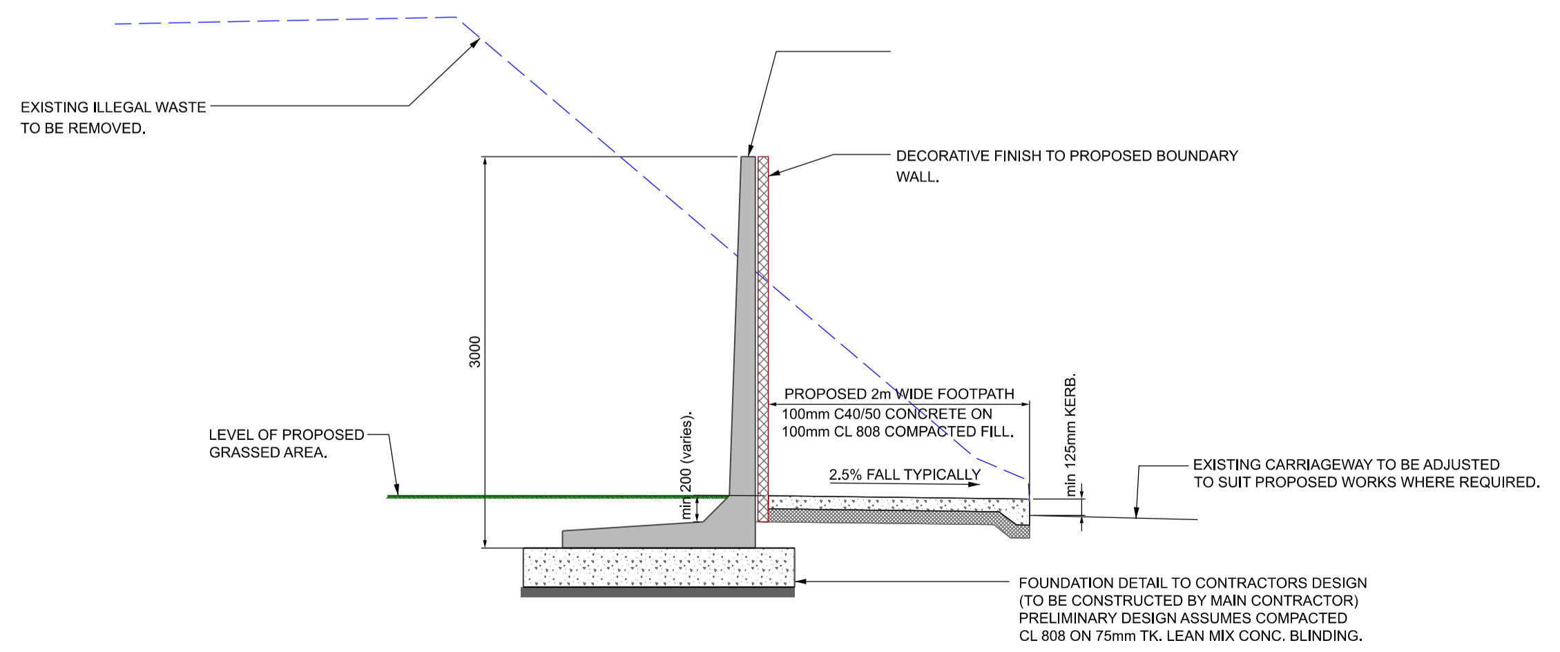
TYPICAL SECTION A - A THRO' PROPOSED BOUNDARY WALL, CHAINAGE 70.0m (approx.) (SCALE 1:20)
