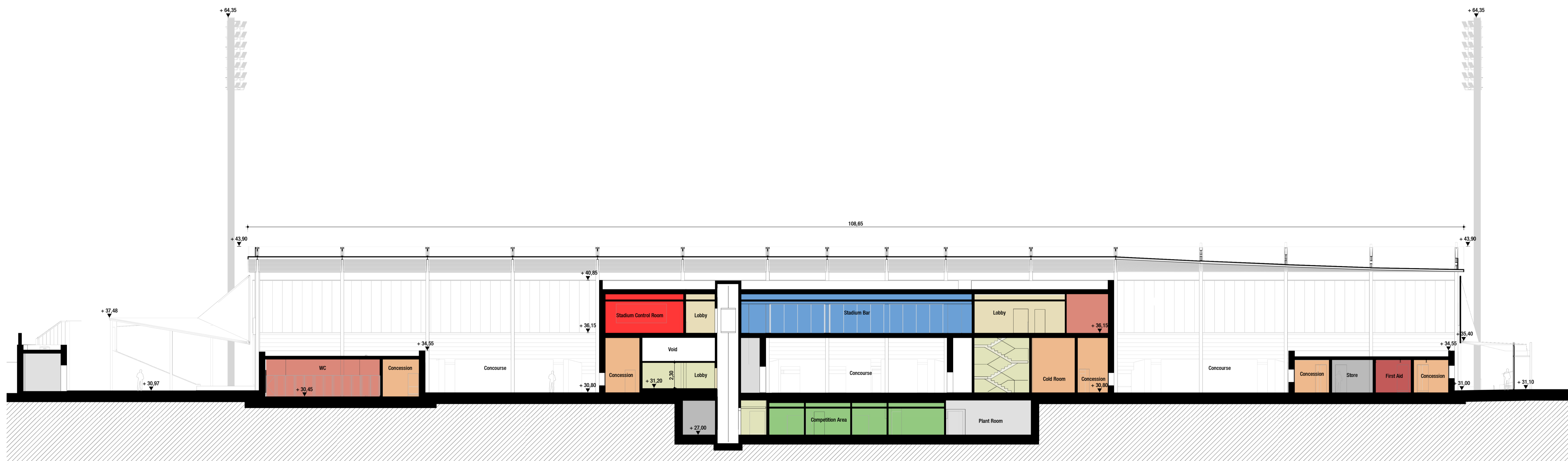
05 Proposed Section 05 Scale 1:200
