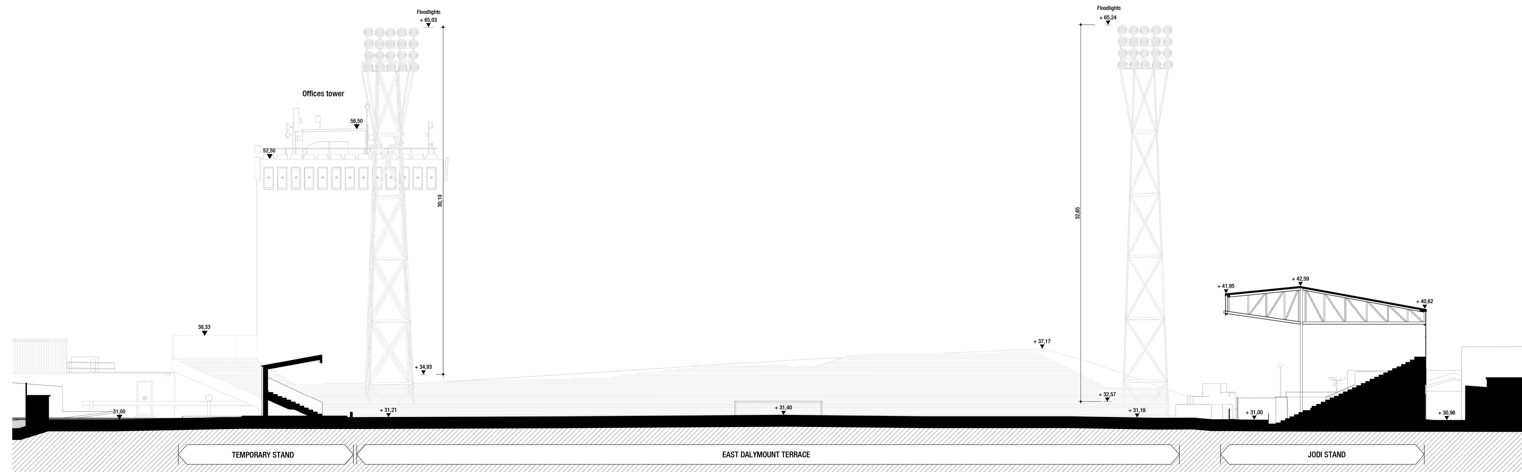
04 Existing GA Section 04 Scale 1:200
