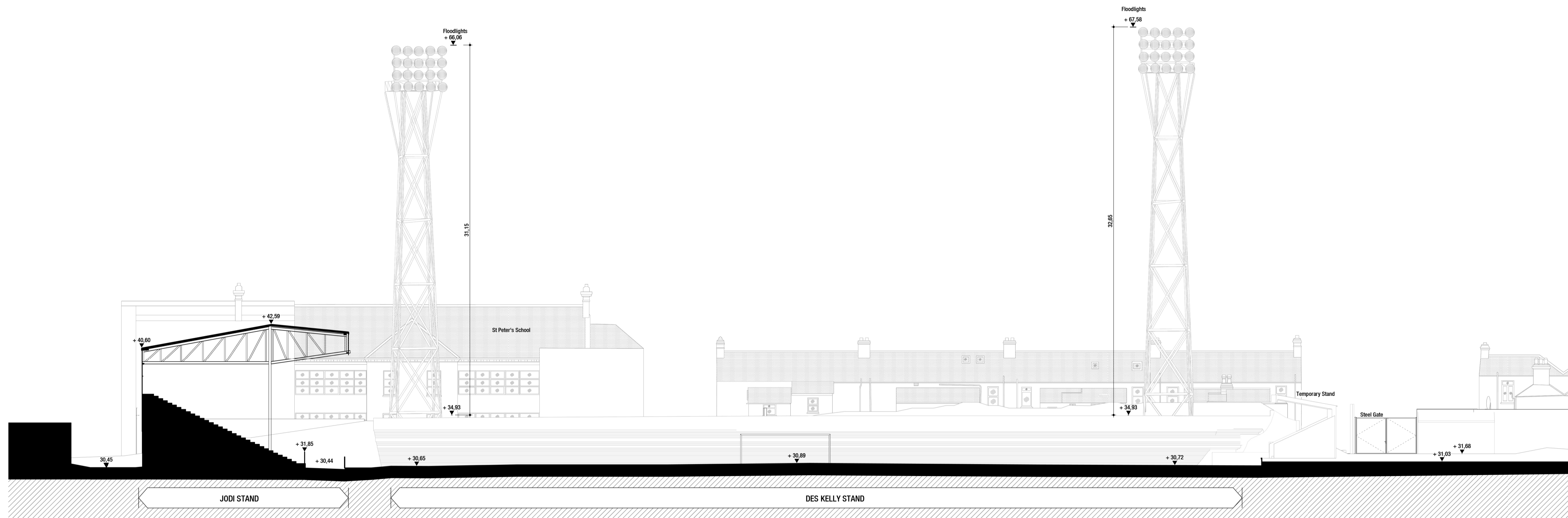
03 Existing GA Section 03 Scale 1:200
