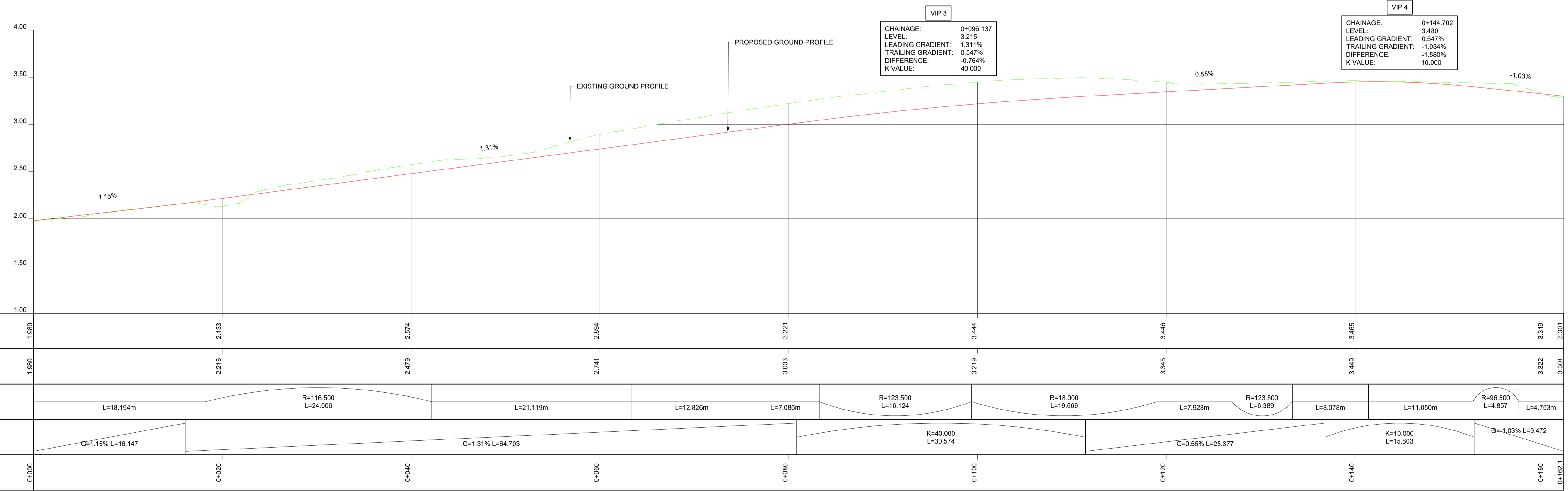
ALIGNMENT - LIBRARY SQ CL PROFILE A1 SCALE: 1:250 HORIZONTAL, 1:25 VERTICAL
