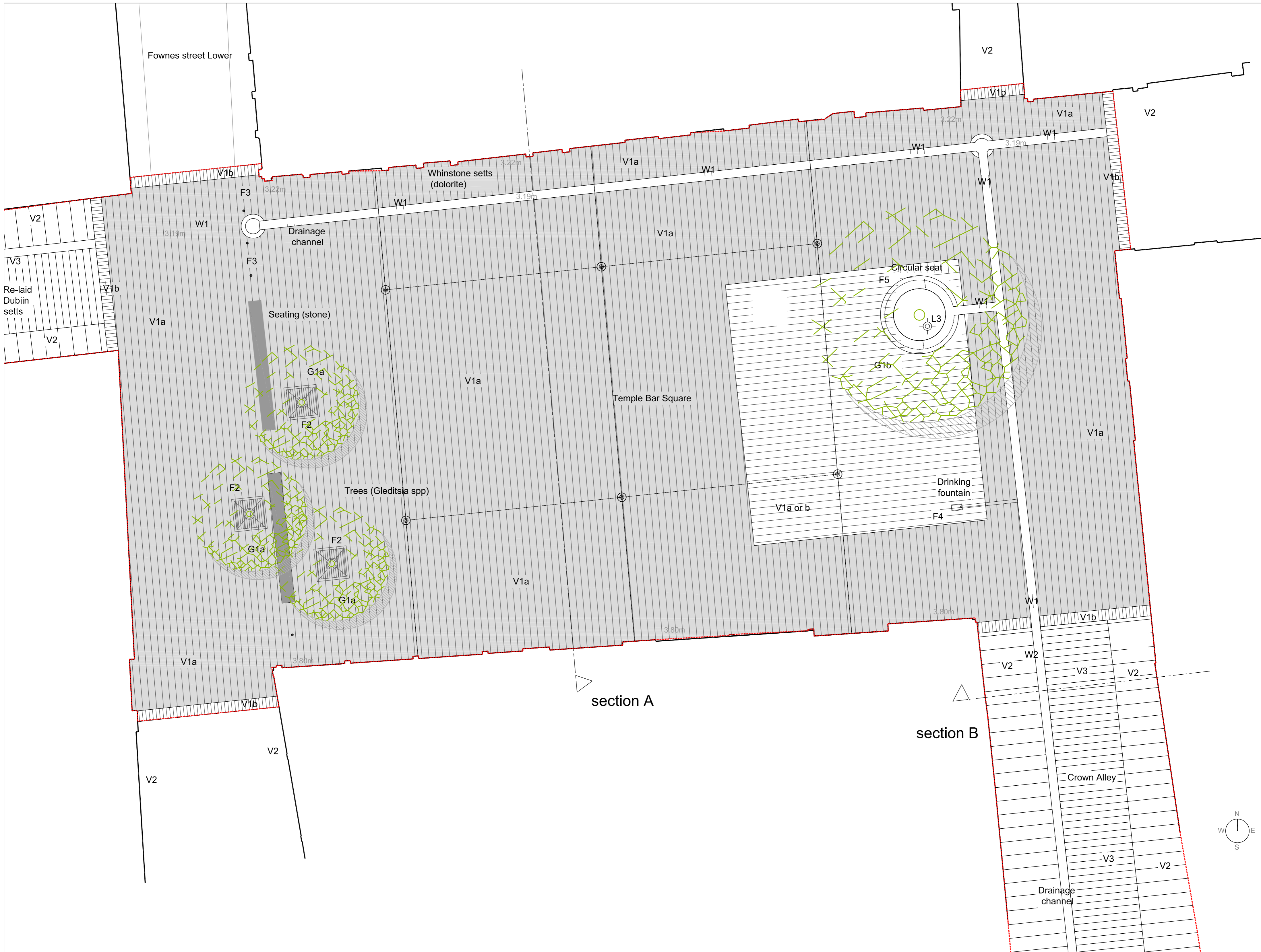
Layout plan 1:100
