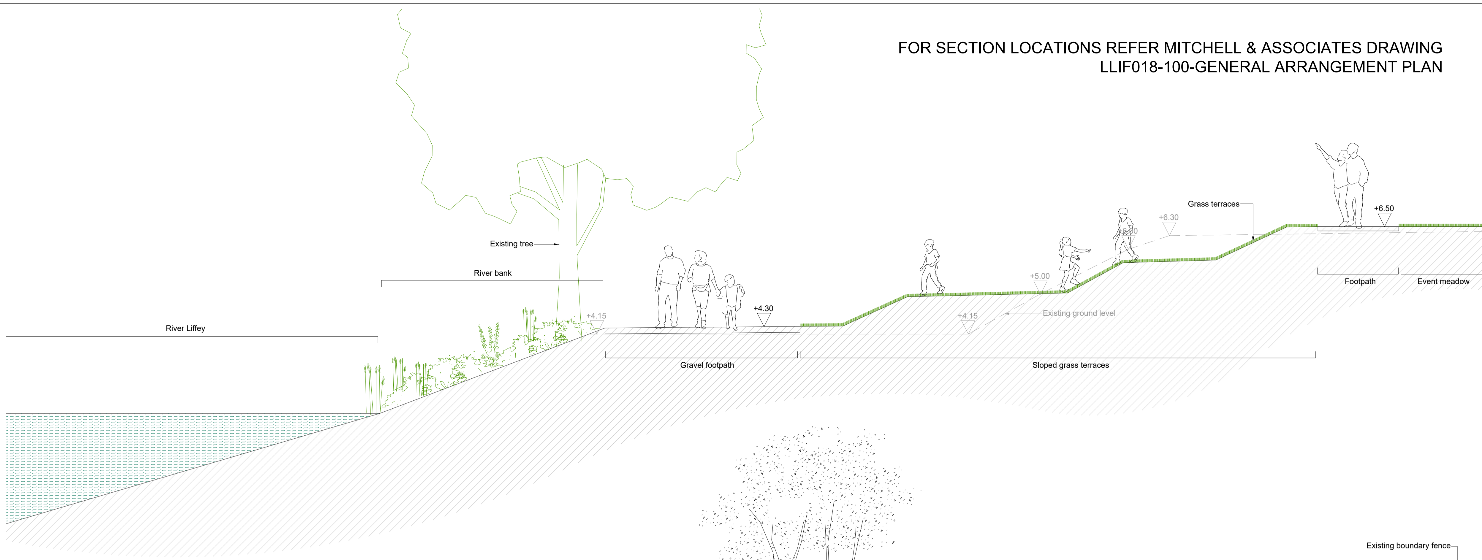
SECTION A-A' Scale 1:50 @A1
