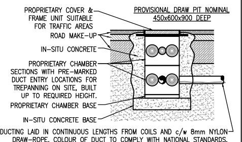
2 DETAIL TYPICAL ACCESS CHAMBER / DRAWPIT DETAIL
