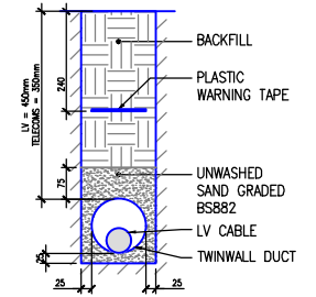
1 DETAIL CABLING IN LAID IN DUCTS ALONG FOOTPATHS
