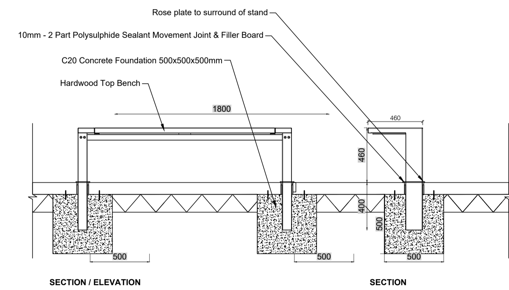
03 Bench / Seat Detail SCALE: 1:20 @ A1
