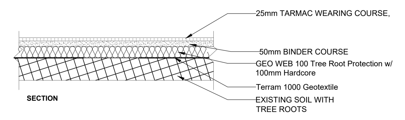
09 PATHS OVER ROOTS SCALE: 1:20 @ A1
