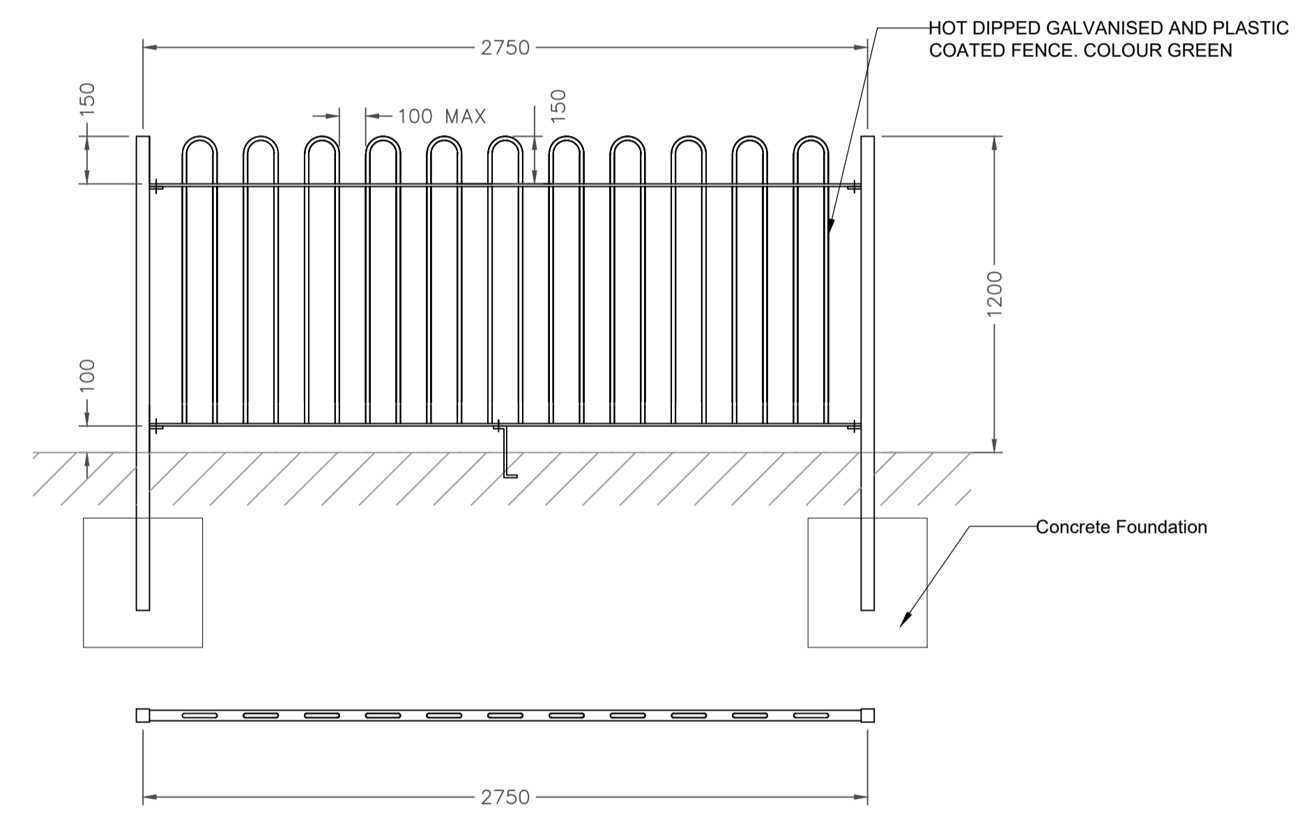
05 BOW TOP FENCE DETAIL (Play Area) SCALE: 1:20 @ A1
