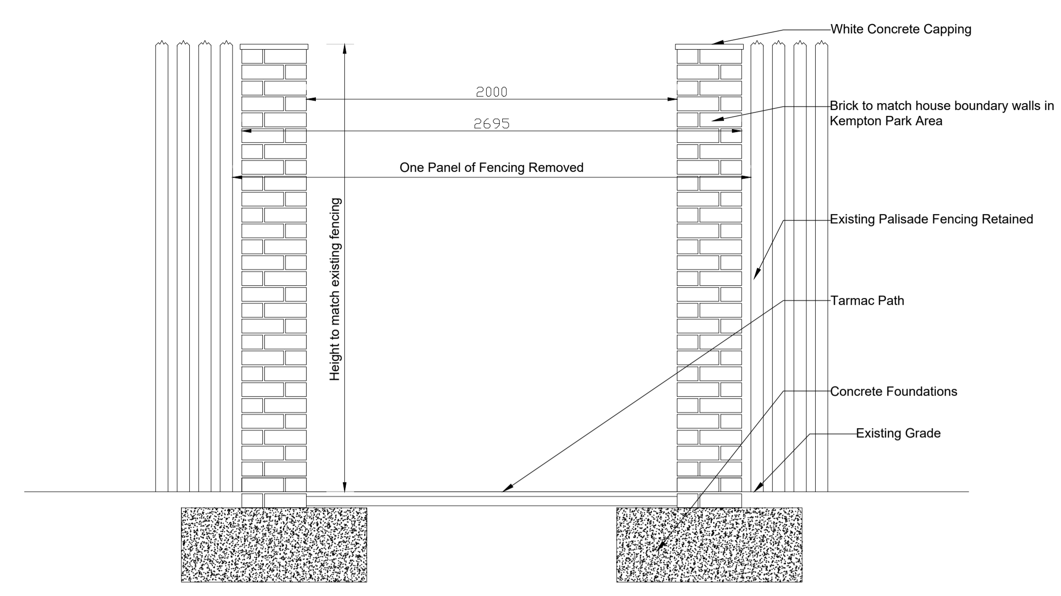
02 PARK ENTRANCE KEMPTON SCALE: 1:20 @ A1
