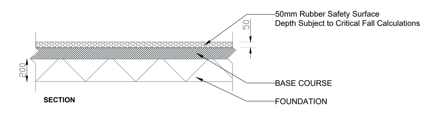
08 SAFETY SURFACE DETAIL SCALE: 1:20 @ A1
