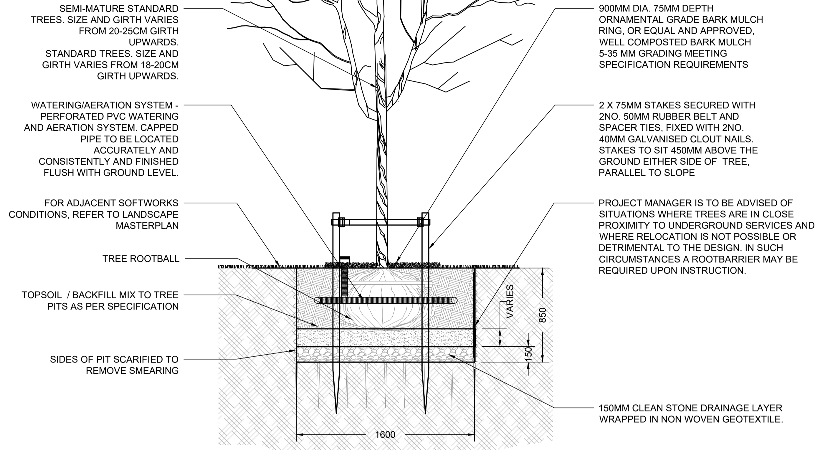
01 TREE PLANTING IN SOFT LANDSCAPED AREAS 7000 SCALE: 1:20 @A1
