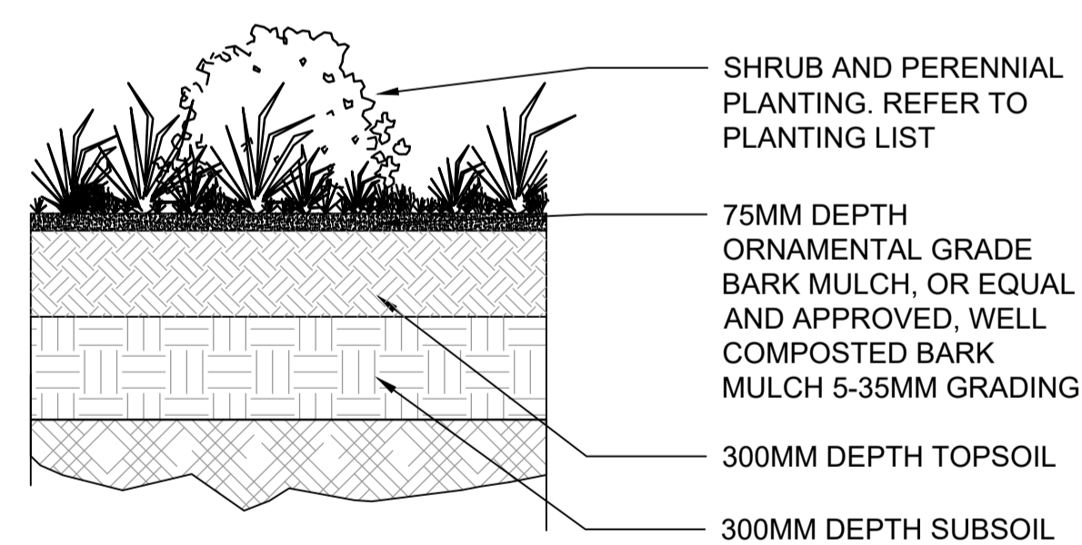
03 SHRUB AND PERENNIAL PLANTING DETAIL 7000 SCALE: 1:20 @A1
