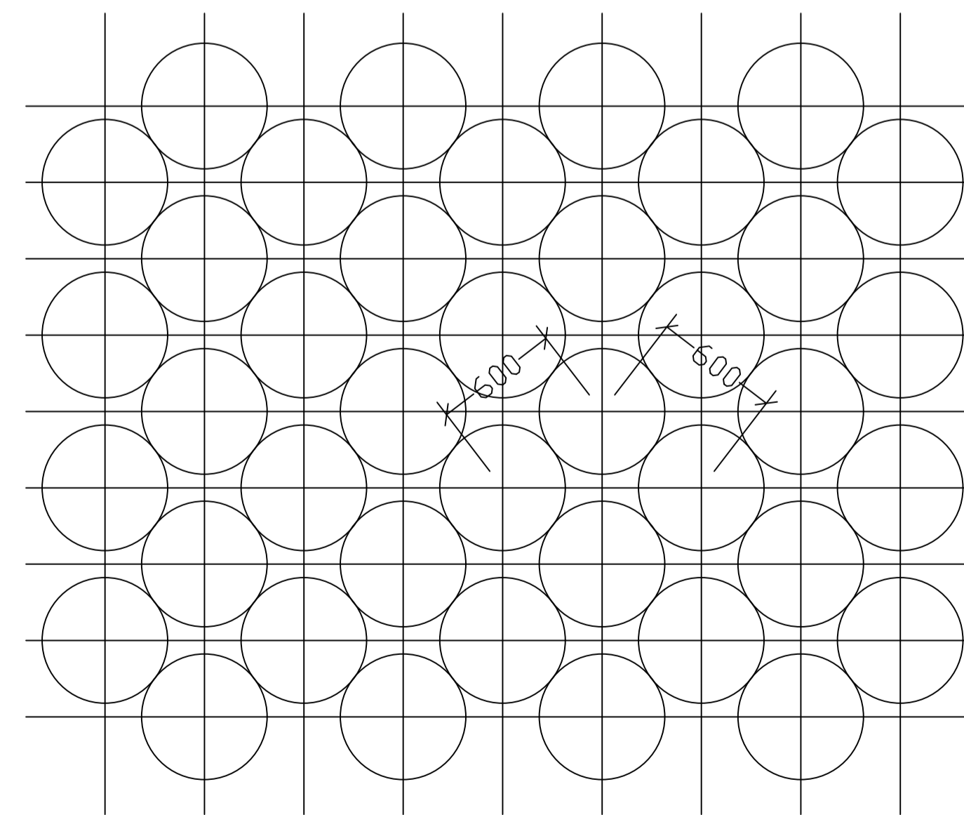
06 SHRUB AND PERENNIAL SPACING CHART 7000 SCALE: 1:20 @A1
