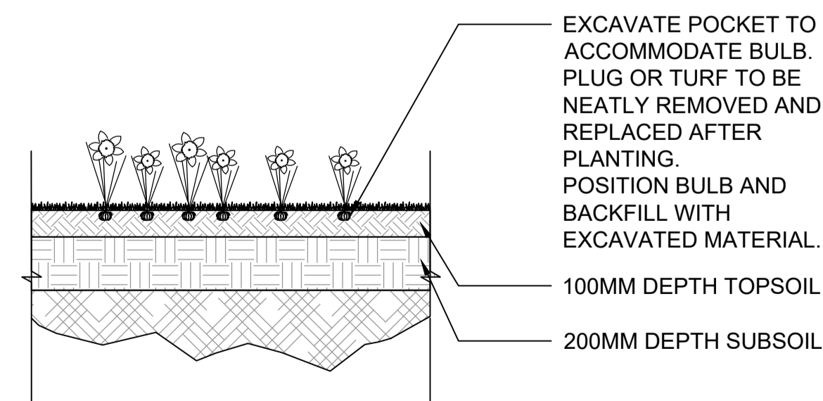
05 TYPICAL PROFILE: BULBS 7000 SCALE: 1:20 @A1
