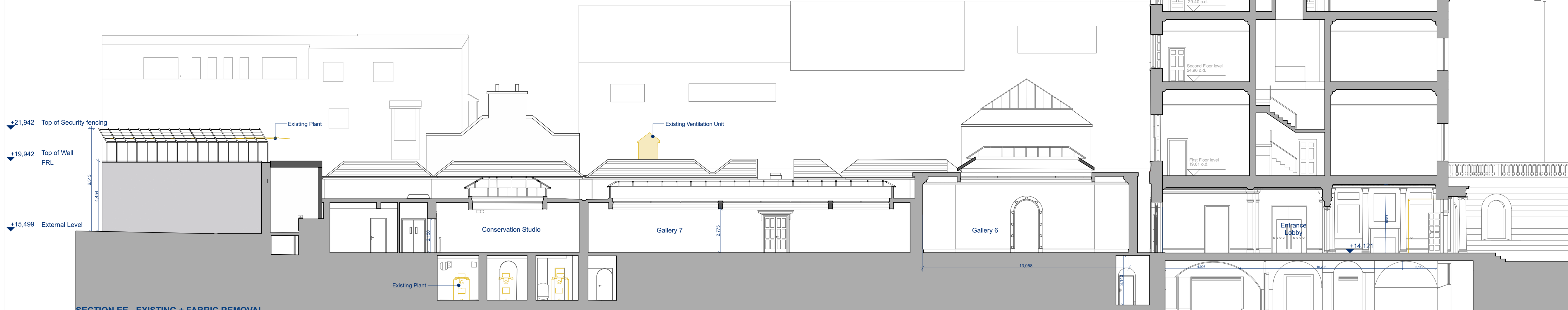
SECTION EE - EXISTING + FABRIC REMOVAL 1:100
