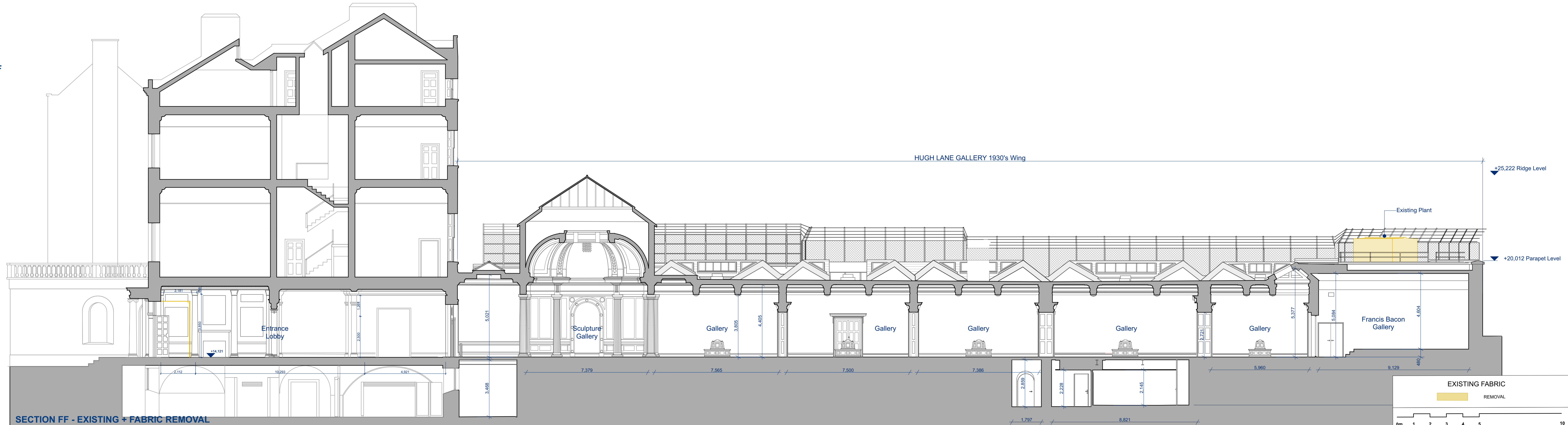
SECTION FF - EXISTING + FABRIC REMOVAL 1:100
