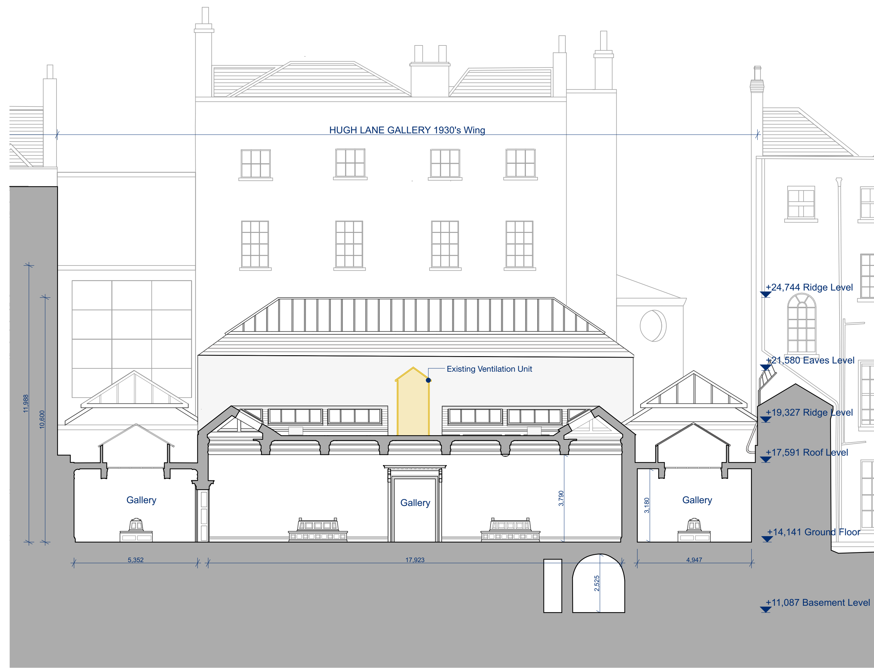
SECTION BB - EXISTING + FABRIC REMOVAL 1:100
