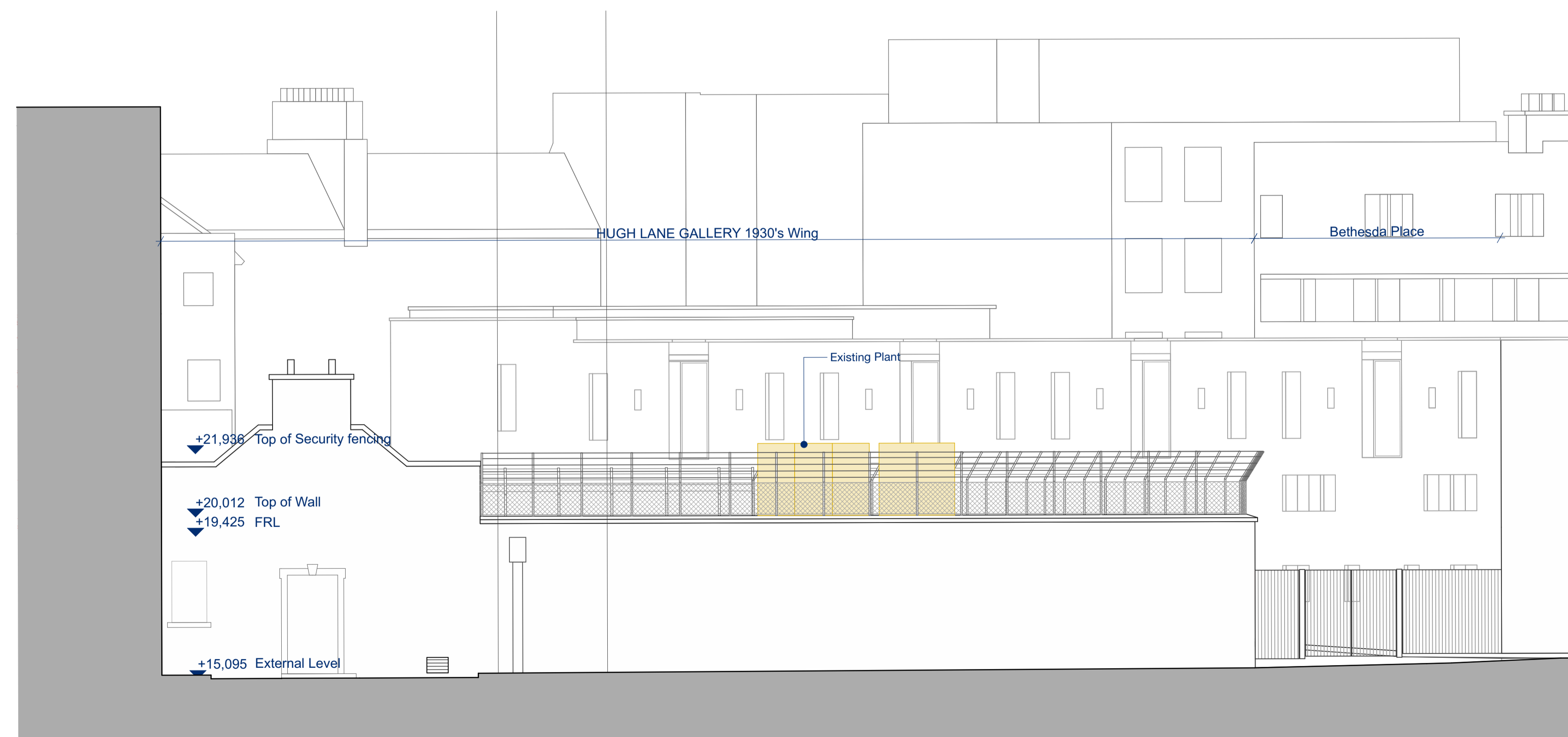
ELEVATION 4 - EXISTING + FABRIC REMOVAL 1:100
