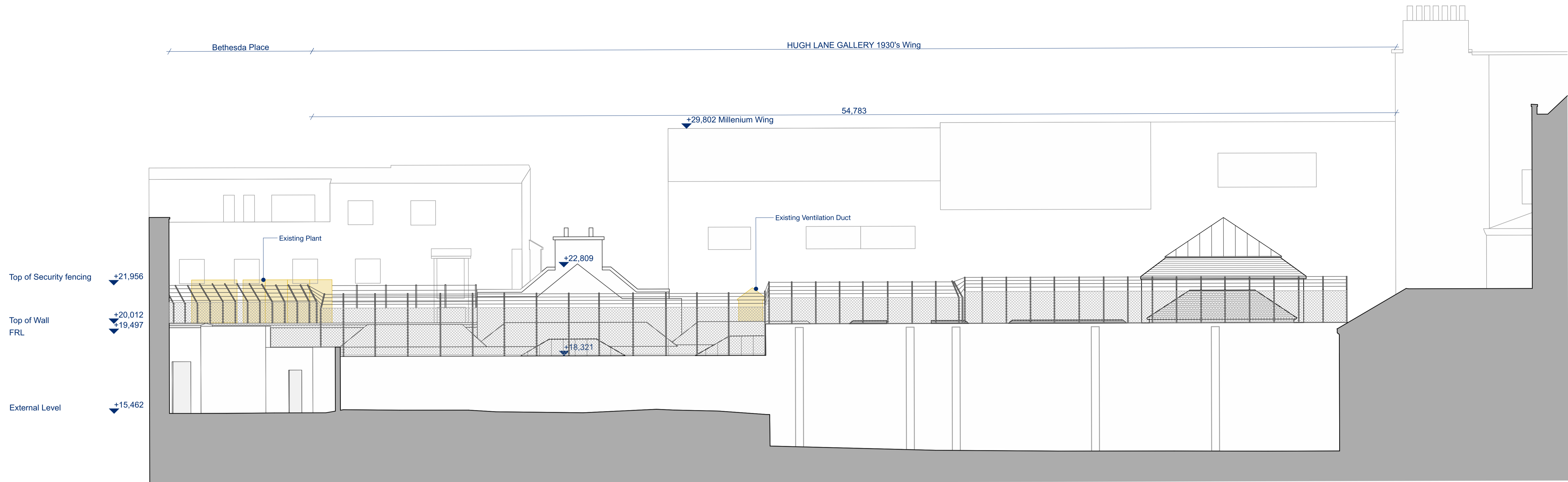
ELEVATION 3 - EXISTING + FABRIC REMOVAL 1:100
