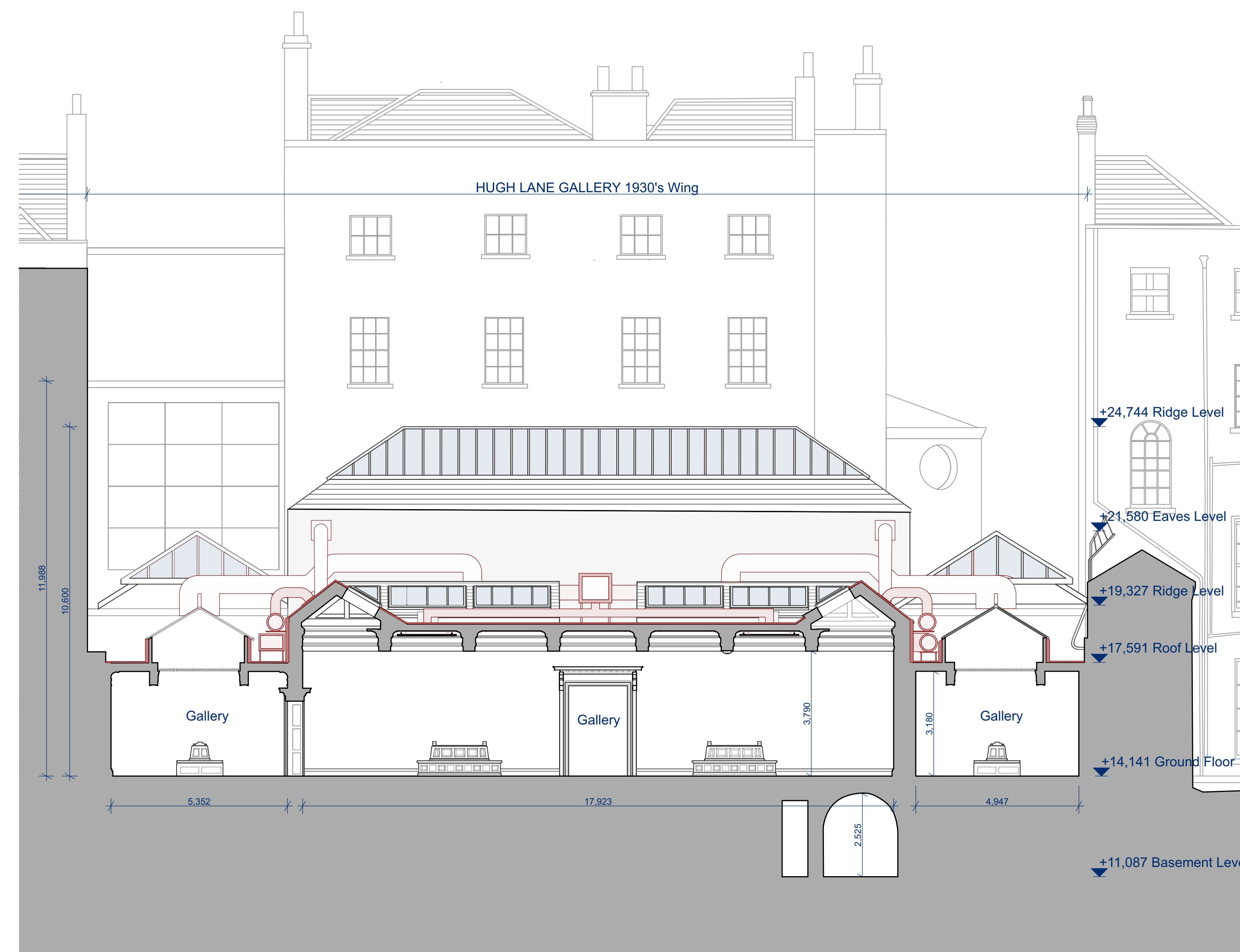
SECTION BB - PROPOSED 1:100
