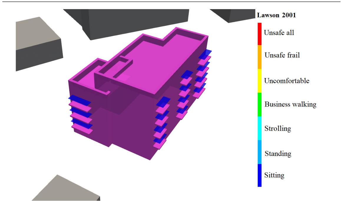
Figure 8.17: Balconies - Lawson Discomfort Map - Proposed scenario
