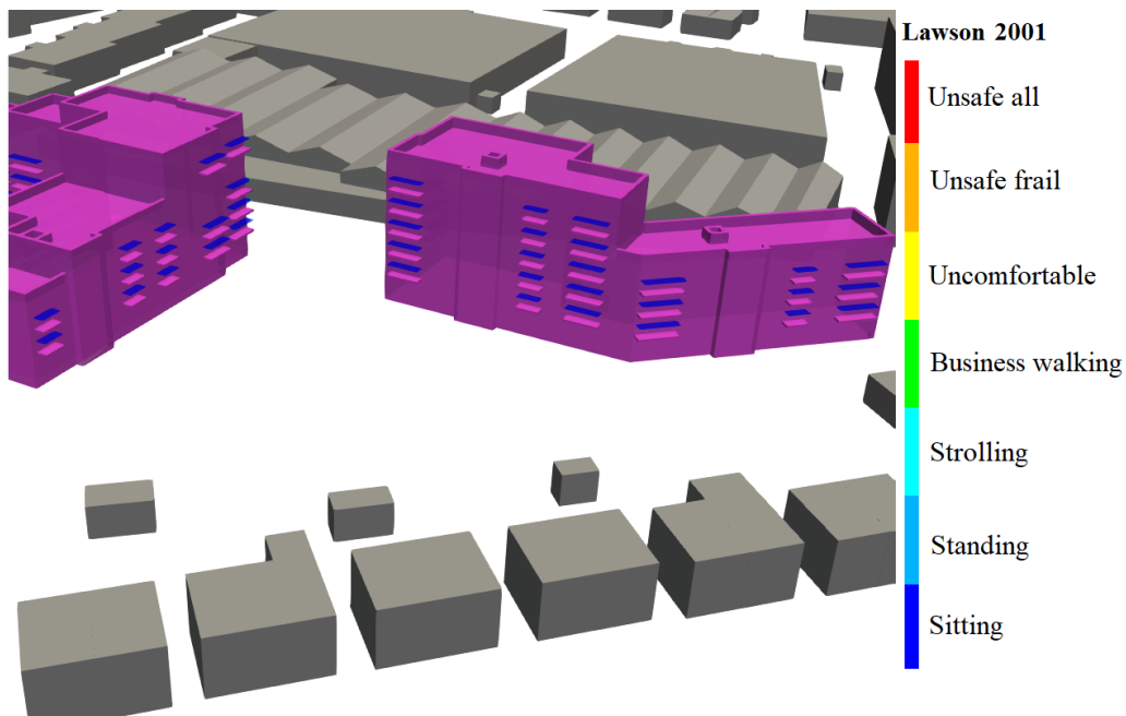
Figure 8.16: Balconies - Lawson Discomfort Map - Proposed scenario
