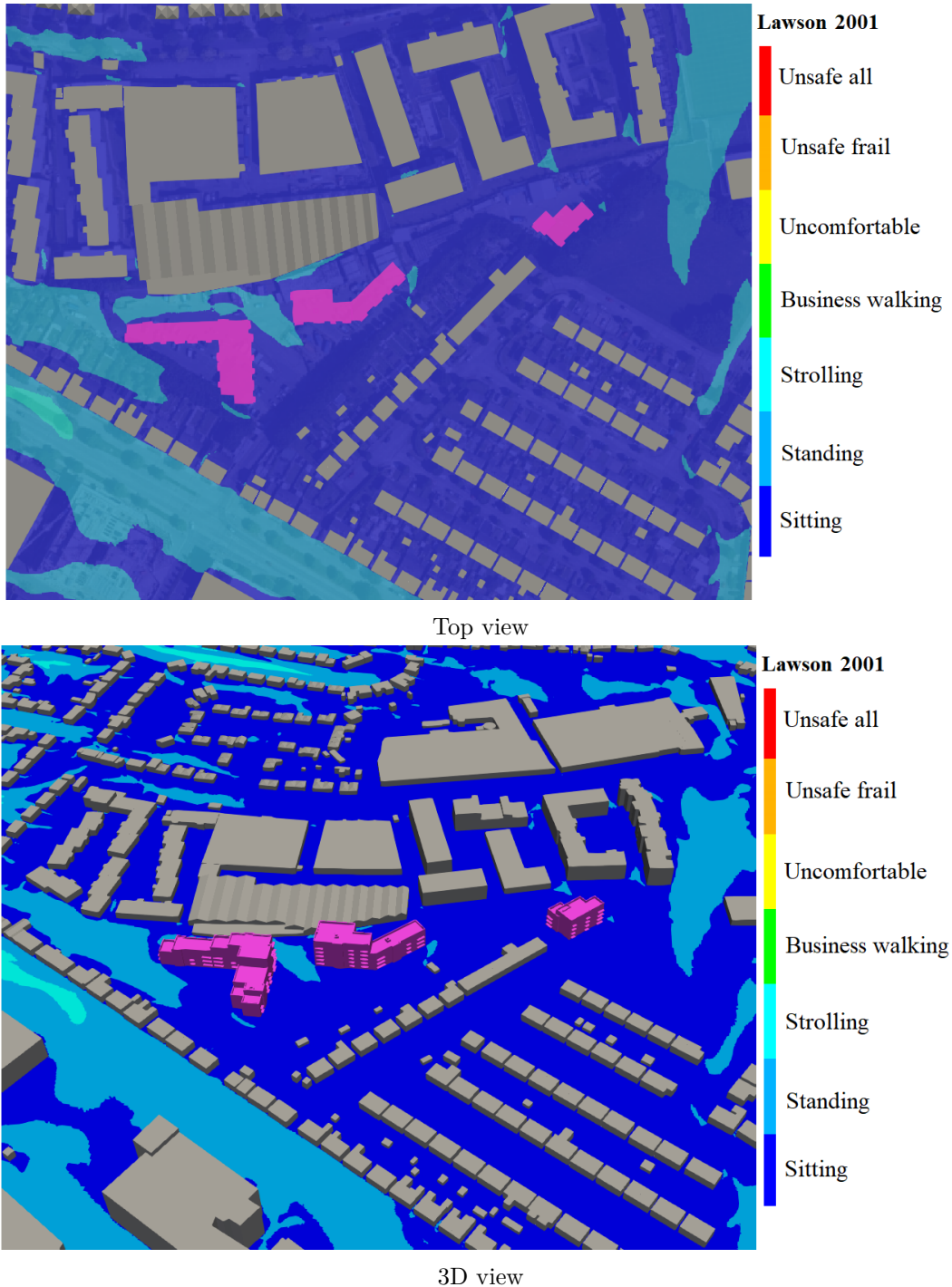
Figure 8.13: Ground Floor - Lawson Discomfort Map - Proposed scenario
