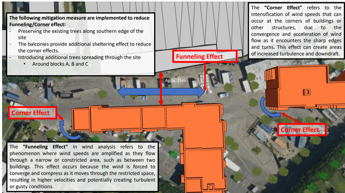
Figure 8.18: Mitigation Measures for Downwash Effect
