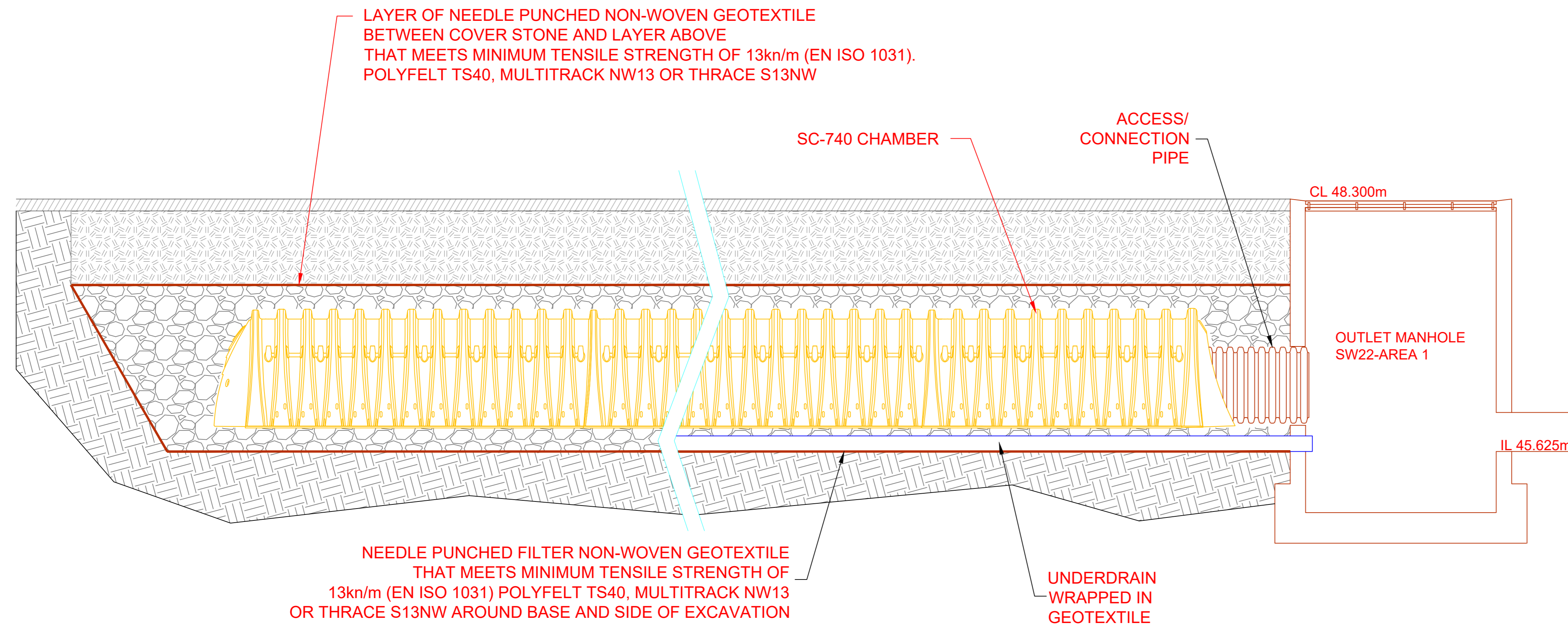
SECTION THRU ATTENUATION TANK - OUTLET MANHOLE SCALE 1:25
