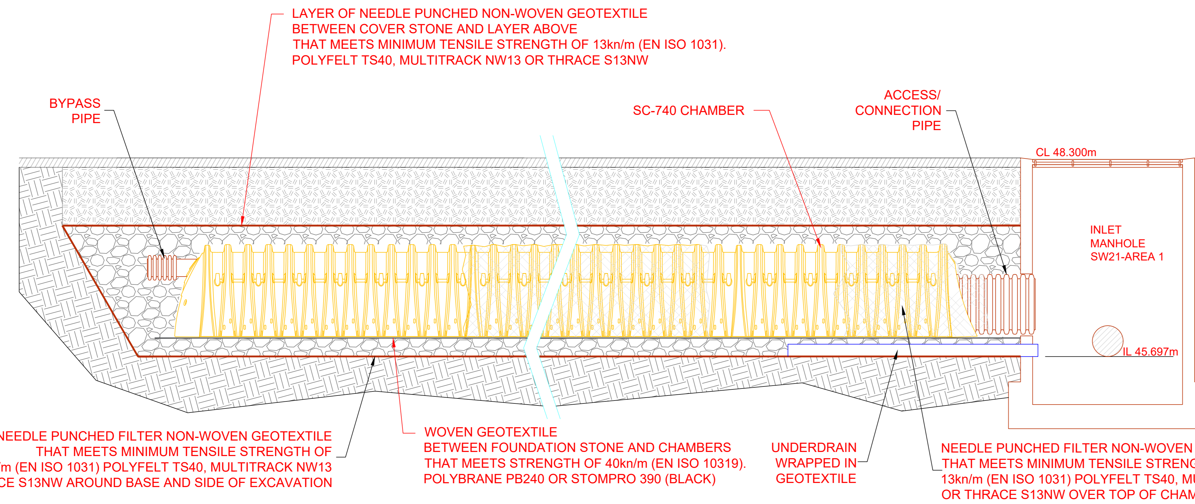
SECTION THRU ATTENUATION TANK - INLET MANHOLE SCALE 1:25
