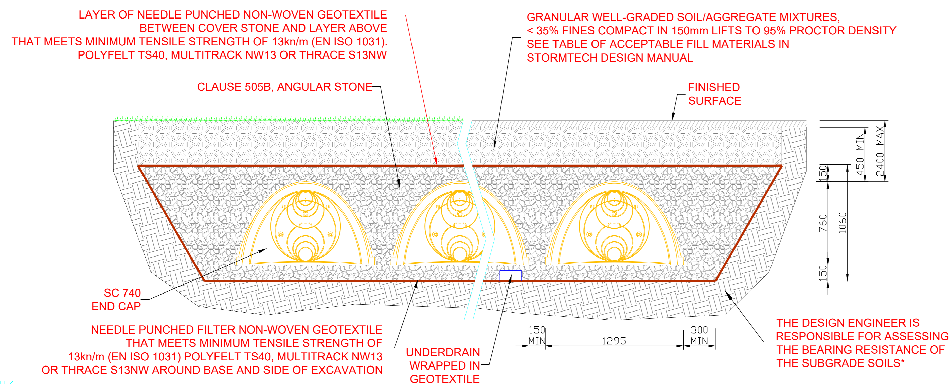
SECTION THRU ATTENUATION TANK - INLET MANHOLE SCALE 1:25
