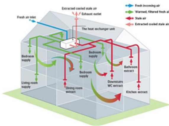
Typical Mechanical Ventilation Heat Recovery (MVHR) Arrangement
