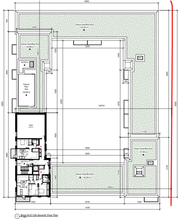
Block B 07-GA- Seventh Floor Plan 1:250
