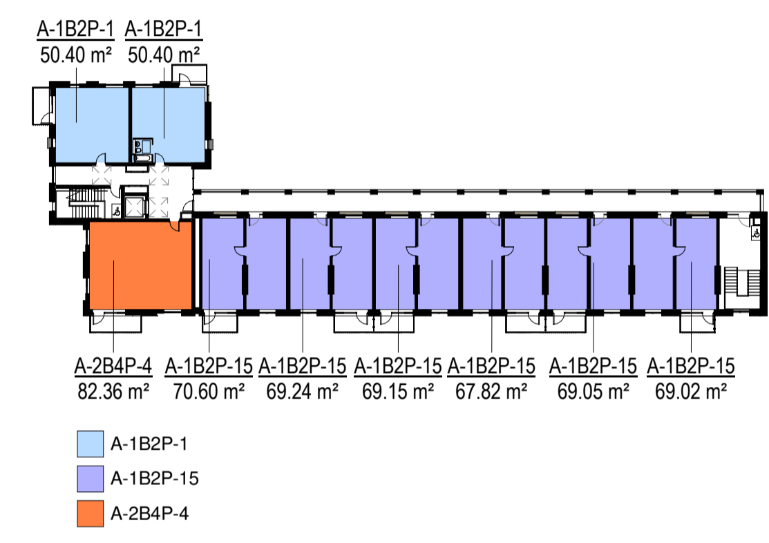
5 Block C - 04 - Fourth Floor - Unit Types 1 : 500
