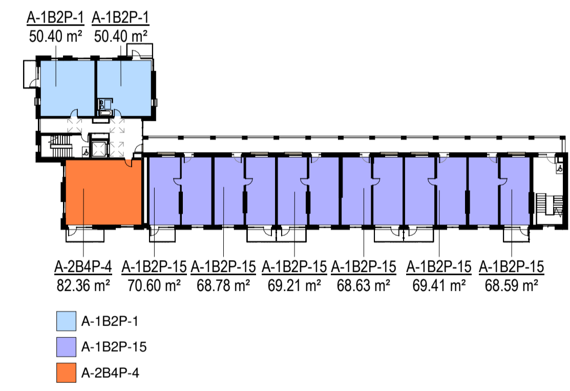
3 Block C - 02 - Second Floor - Unit Types 1 : 500
