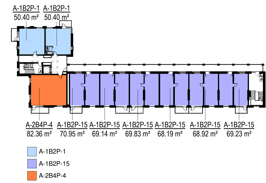
4 Block C - 03 - Third Floor - Unit Types 1 : 500
