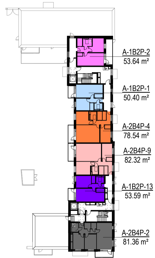
2 Block A - 01 - First Floor - Unit Types 1:500
