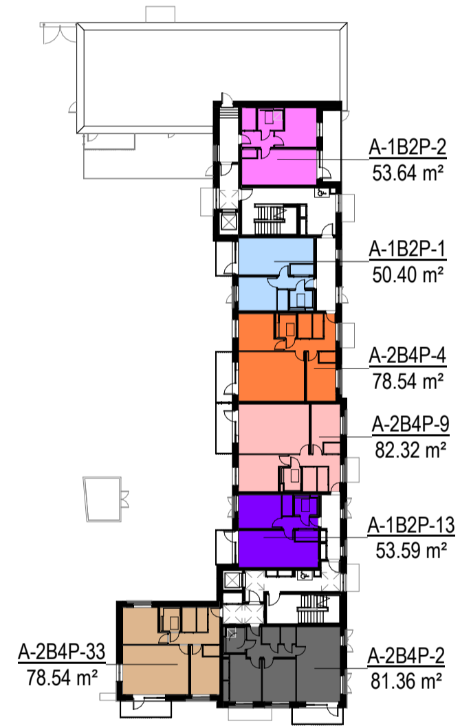
1 Block A - 00 - Ground Floor - Unit Types 1:500
