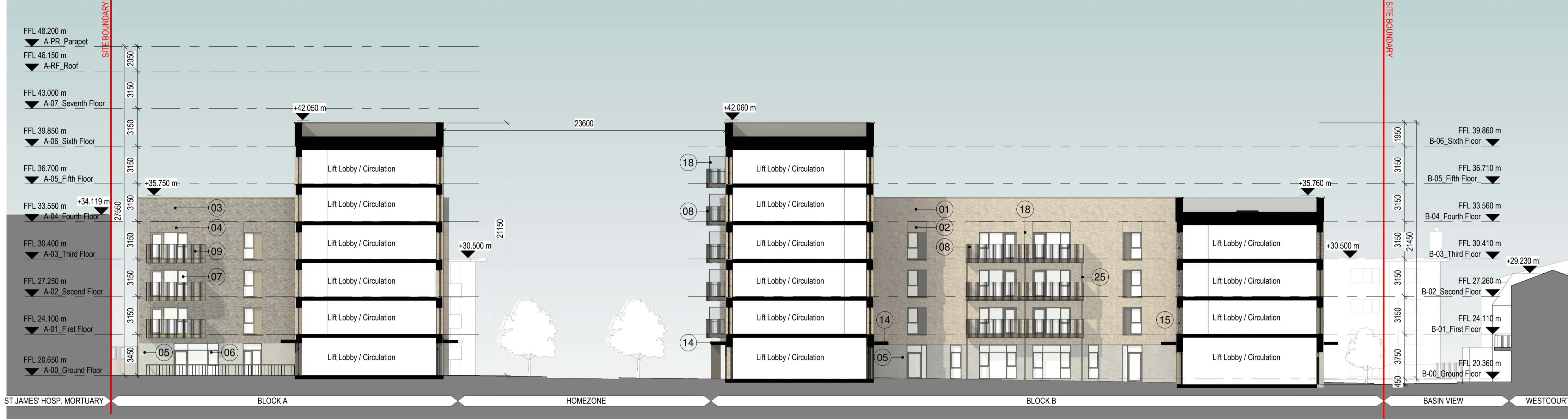
1 Section A-A - Block A & B 1:200
