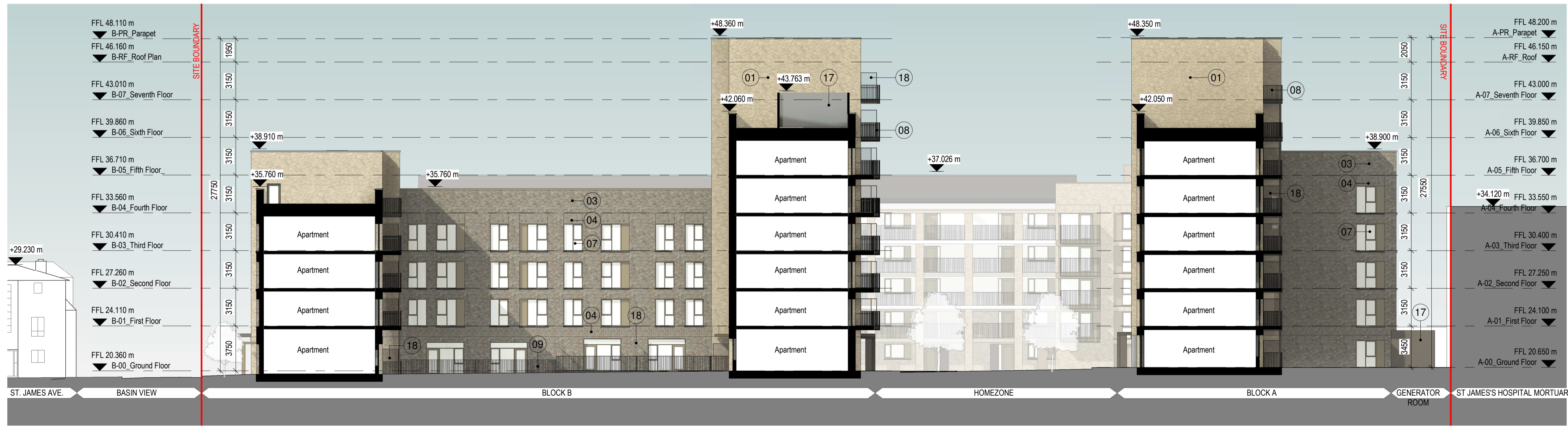
2 Section B-B - Block A & B 1:200
