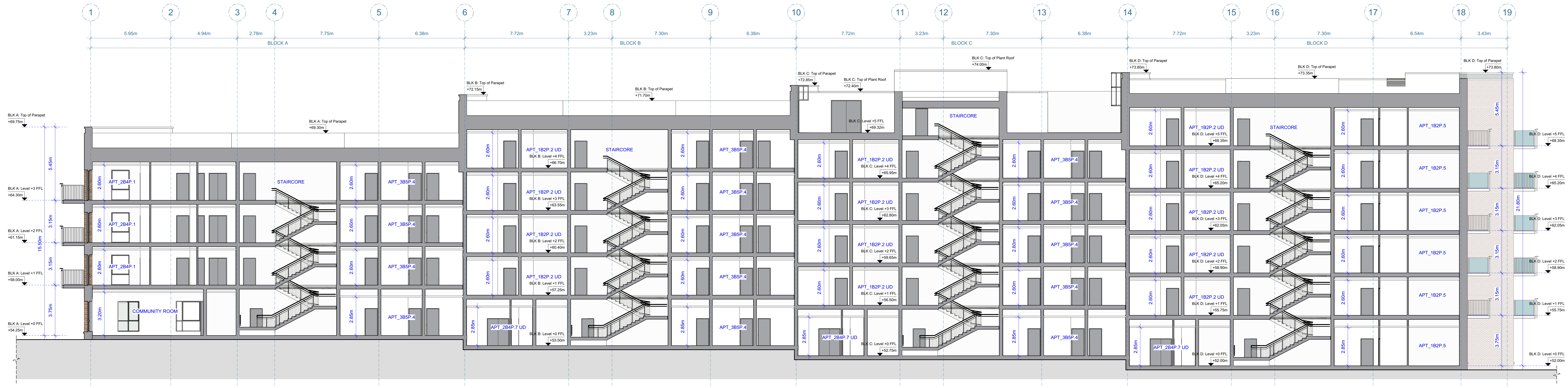
1 Proposed Building Section Scale: 1:100
