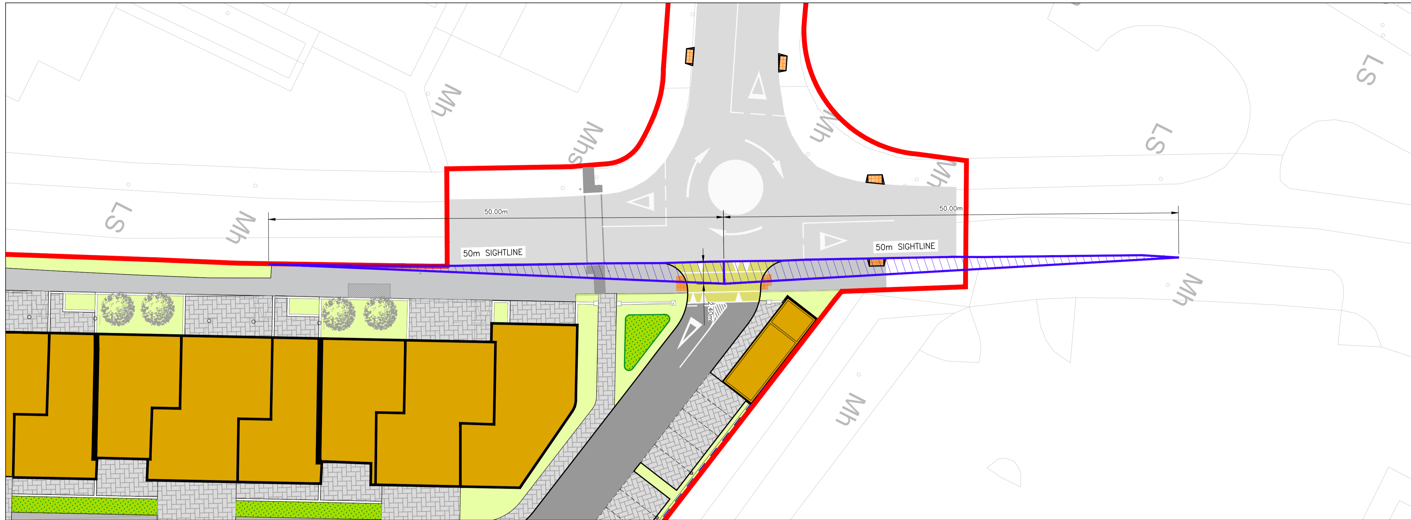
PLAN OF SIGHTLINES FOR JUNCTION WITH CARDIFFSBRIBE ROAD SCALE 1:250
