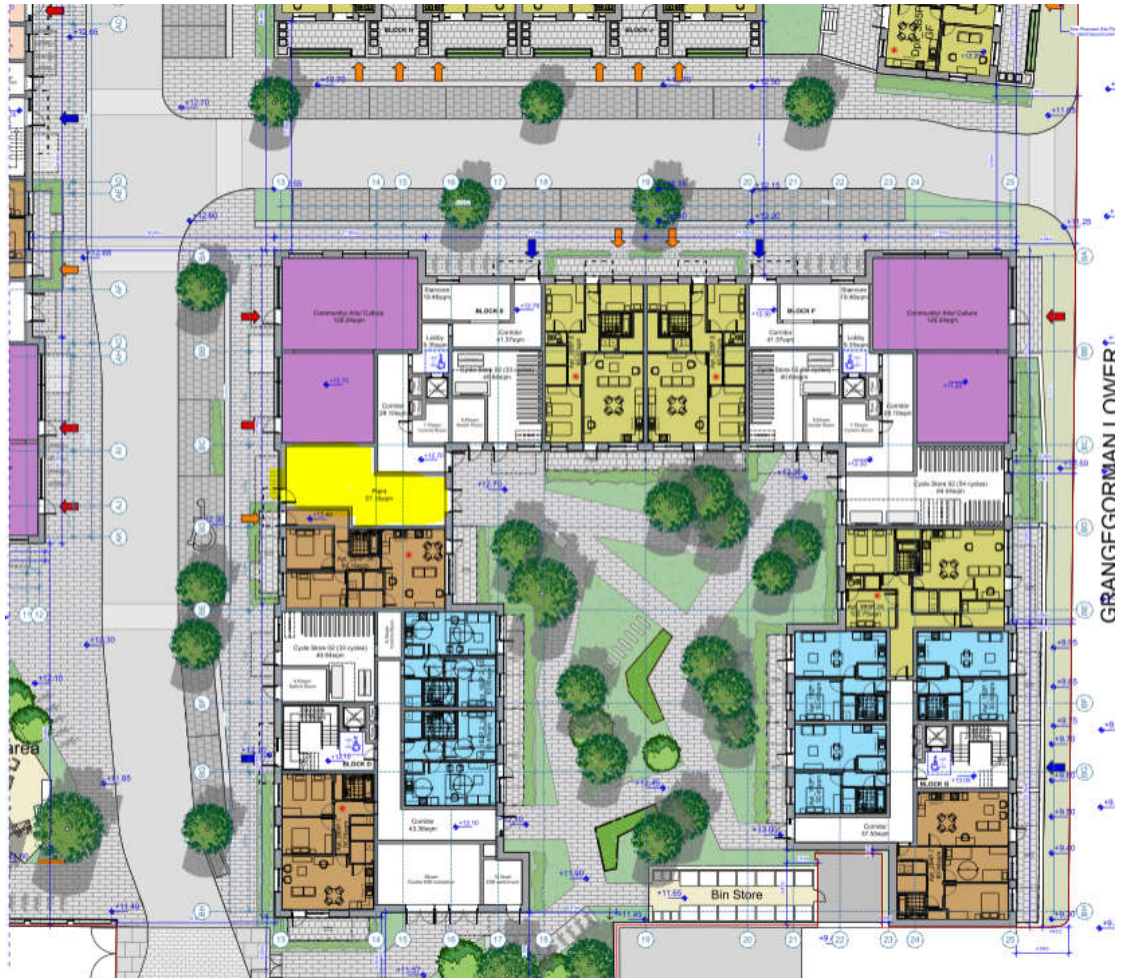
South East Block Ground Floor
