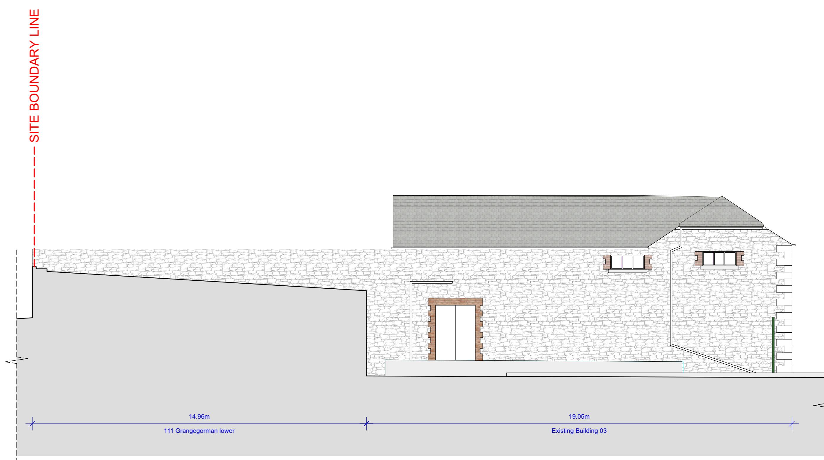
4 Existing Site Section Scale: 1:100
