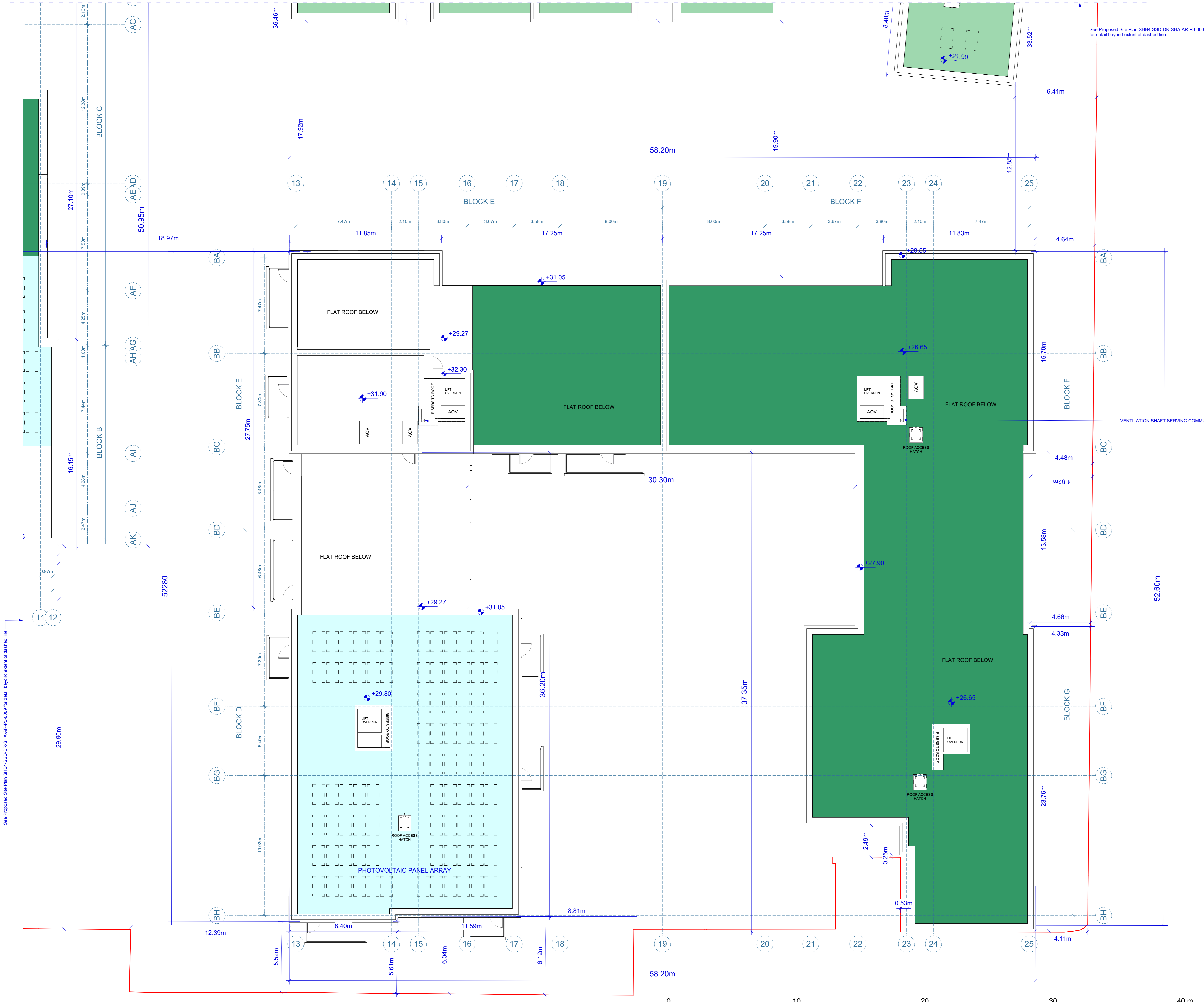
Proposed Roof Level Plan Scale: 1:100
