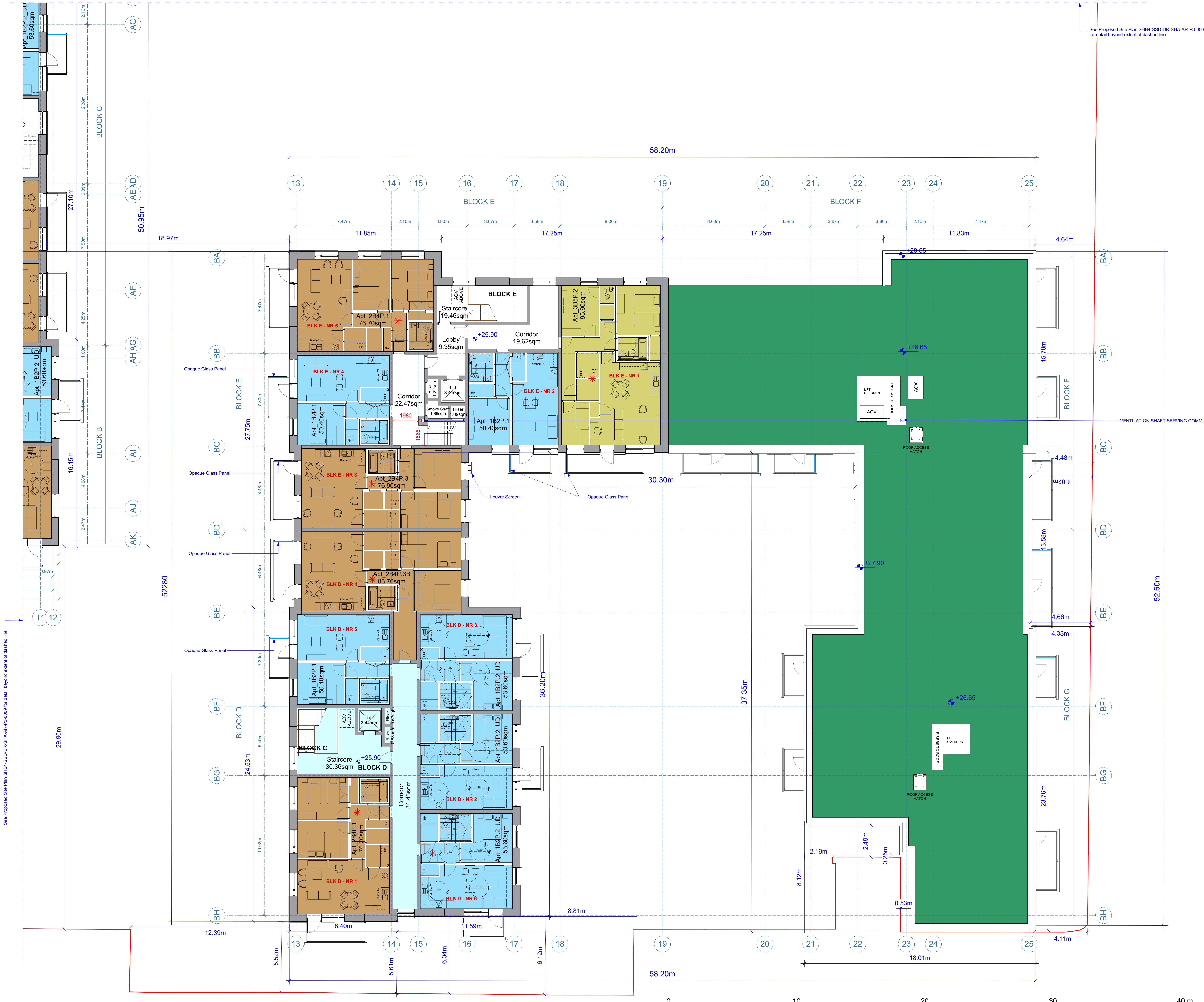
Proposed Level +4 Plan Scale: 1:100
