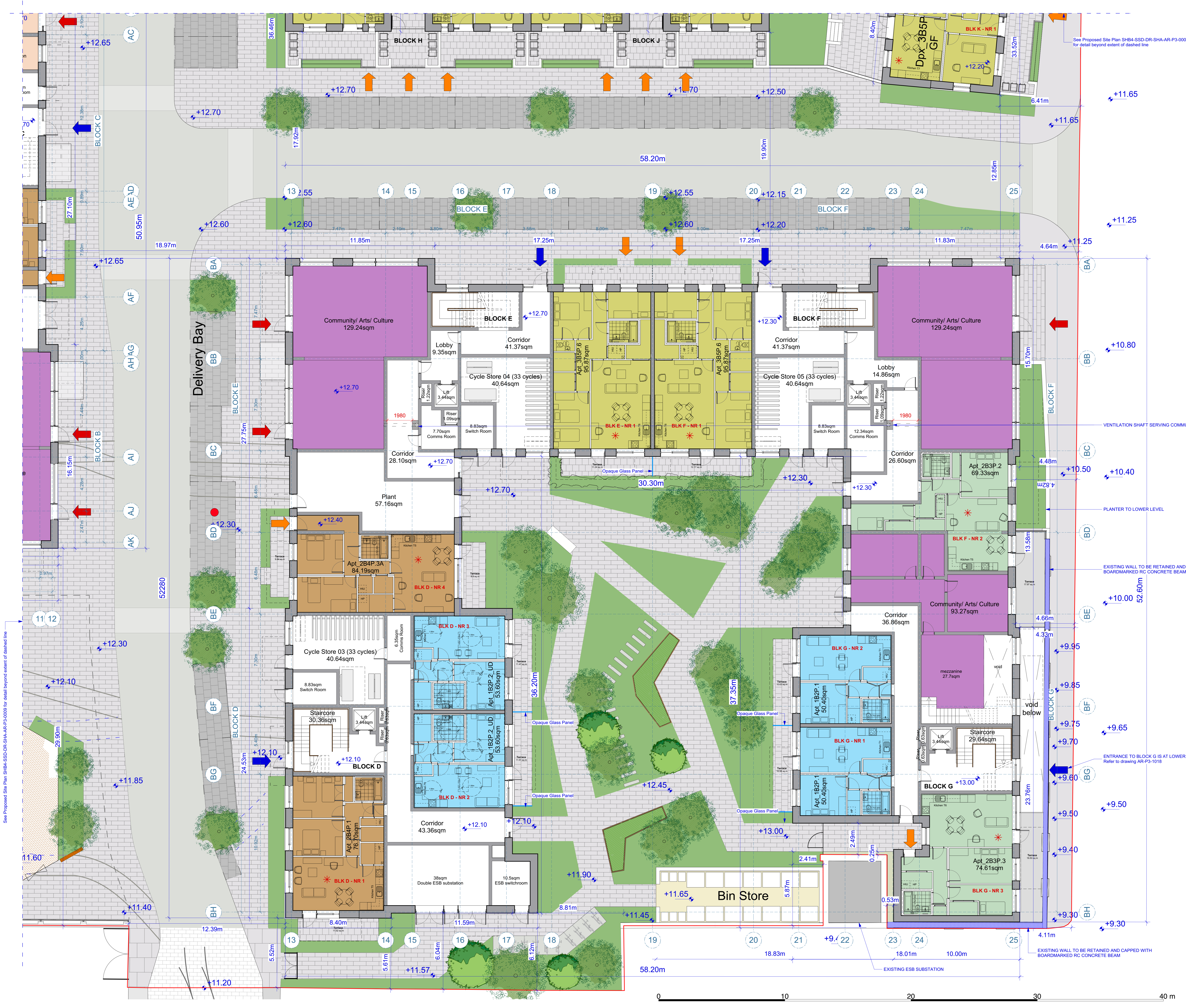
Proposed Level +0 Plan Scale: 1:100
