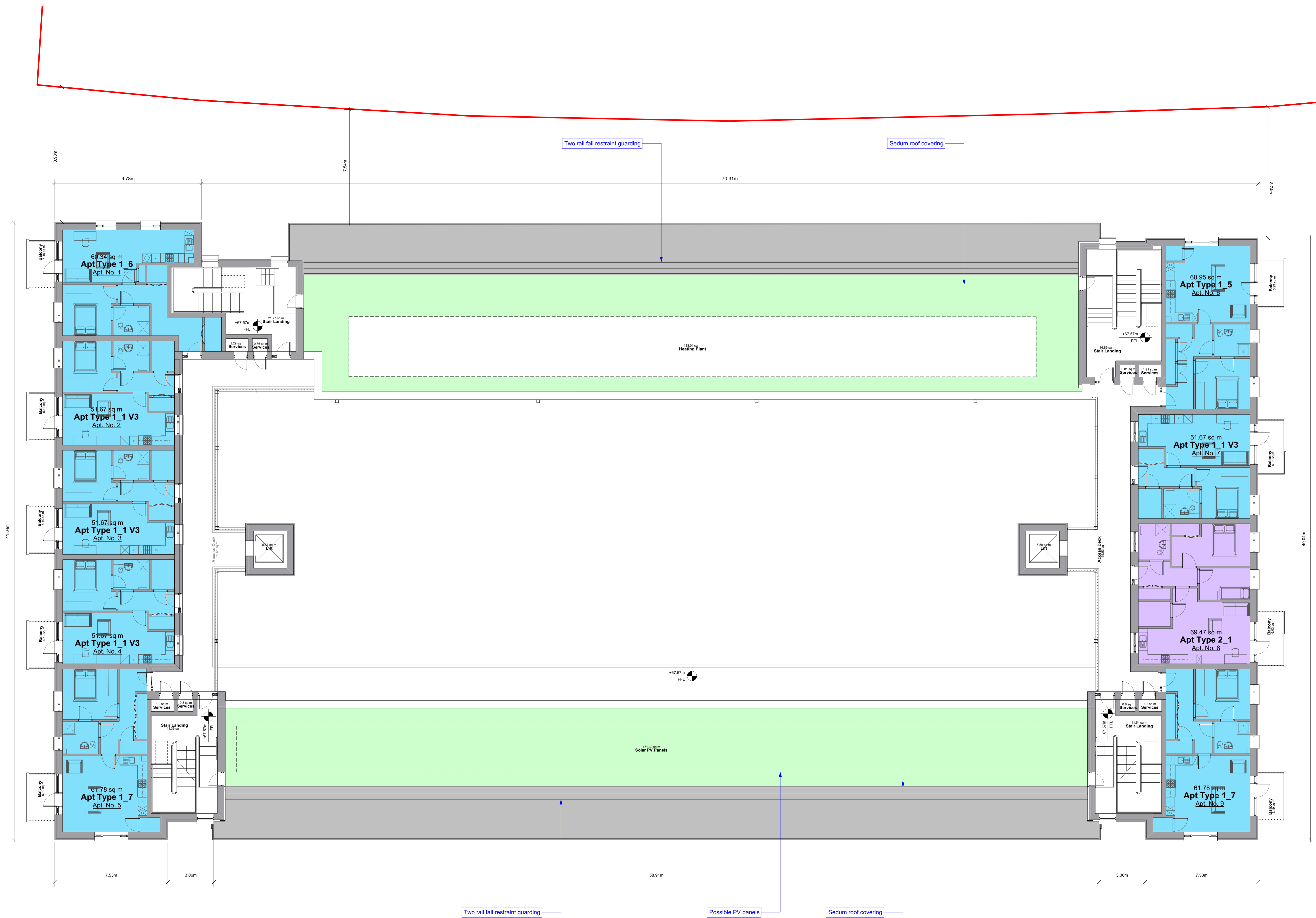
1 Floor Plan - Level +3 Scale: 1:100
