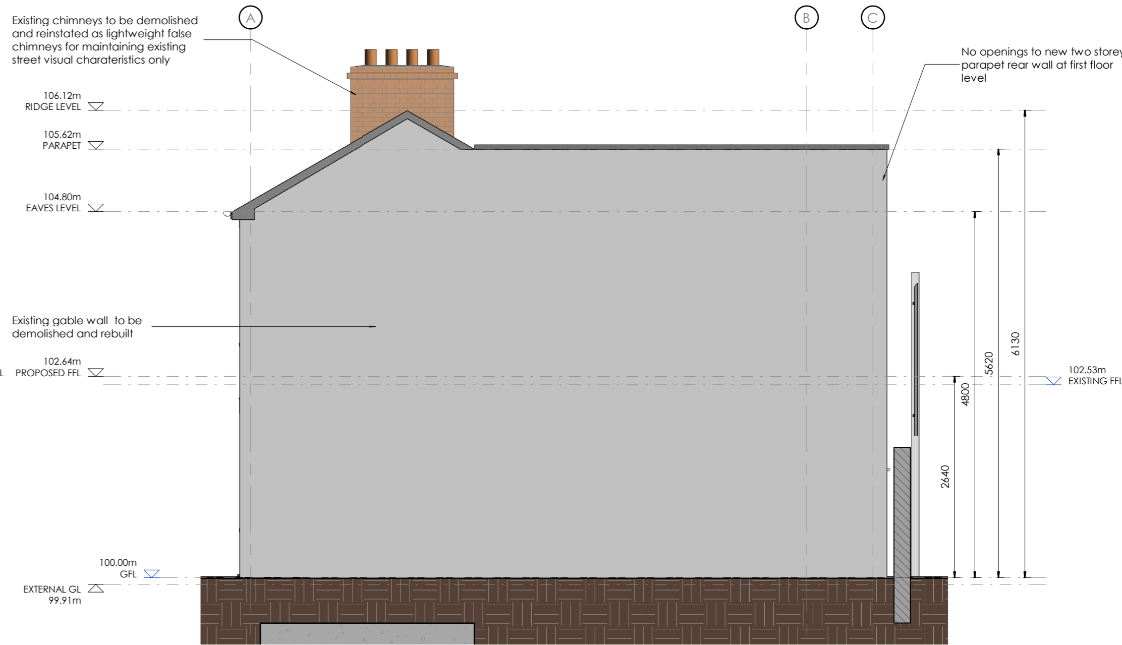
2 Proposed North East Elevation 1 : 50
