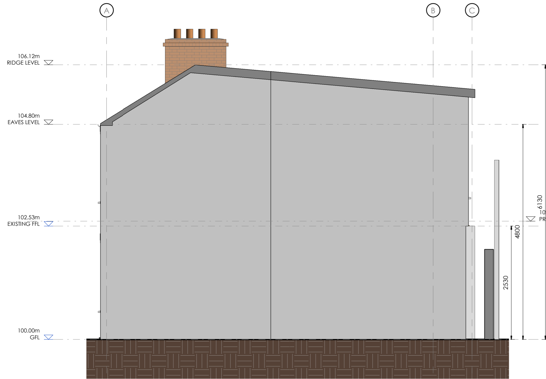
1 Existing North East Elevation 1 : 50
