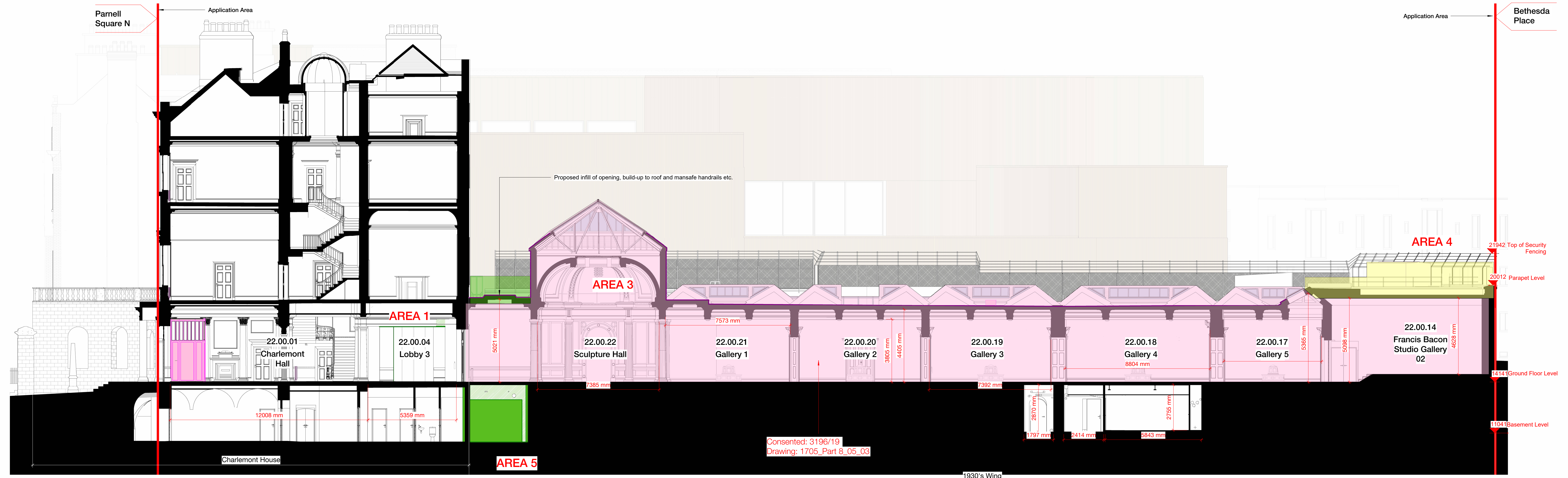
Proposed - Section F-F 1 : 100
