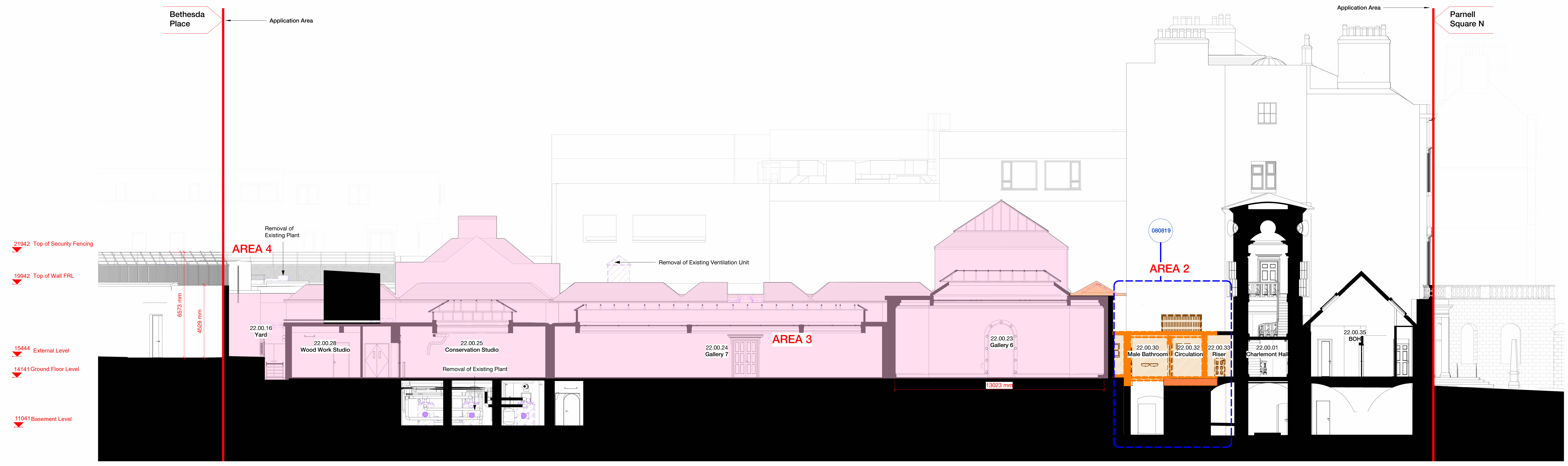
Existing & Fabric Removal - Section E-E 1 : 100
