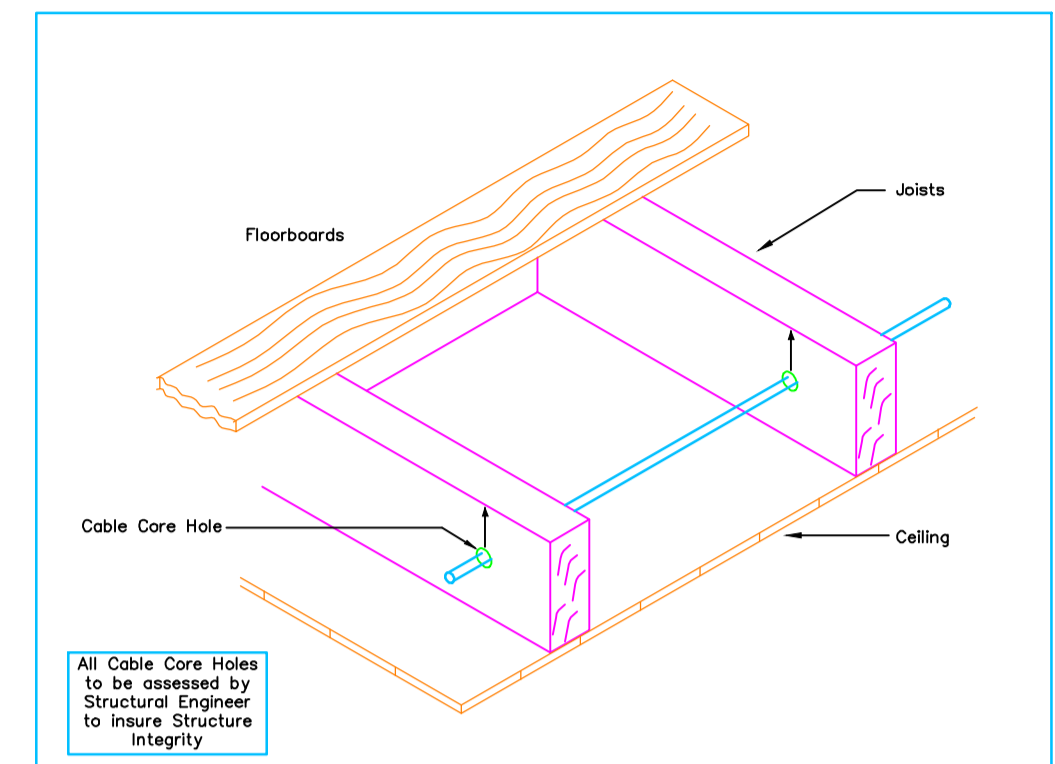
Detail A – Typical Cable Installation through Floor Joists by Coring
