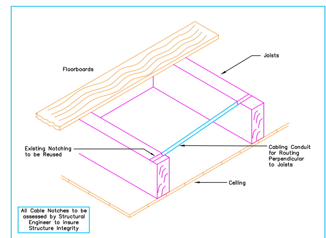
Detail B – Typical Cable Installation through Floor Joists by Notching
