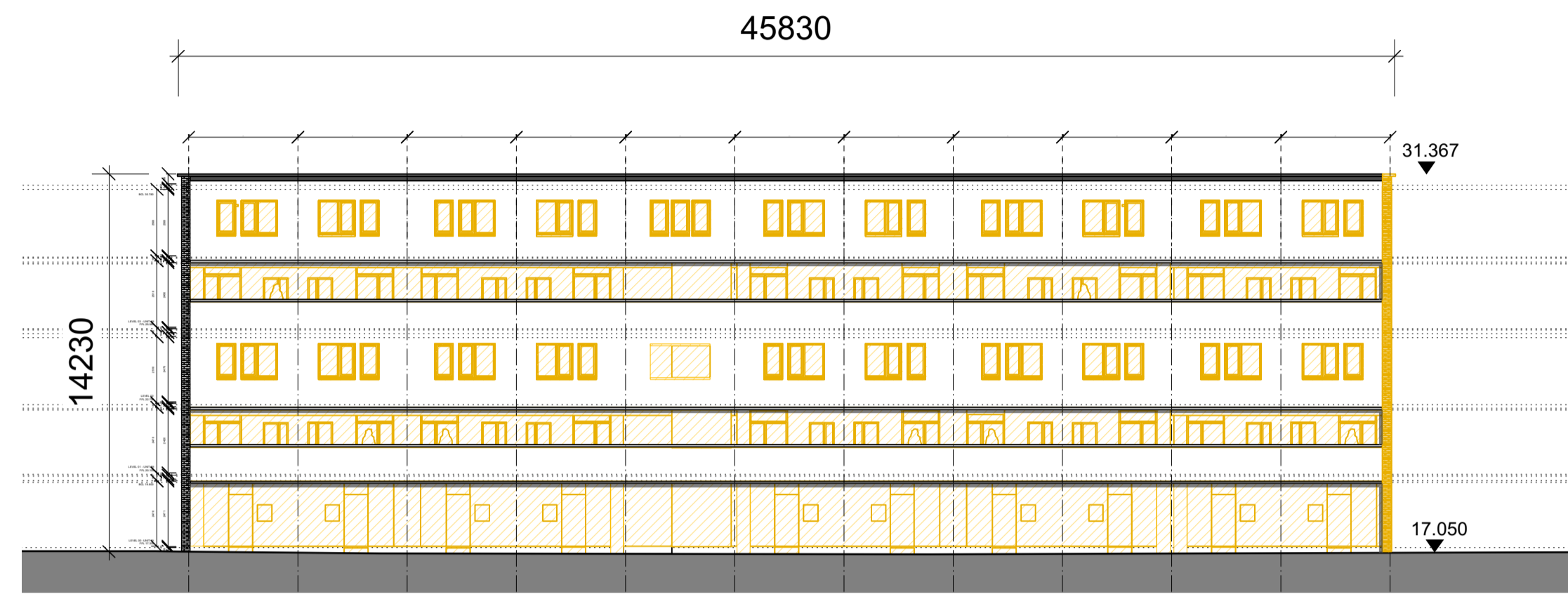
1 Existing And Demolition West Elevation 030204 1:200 @ A1
