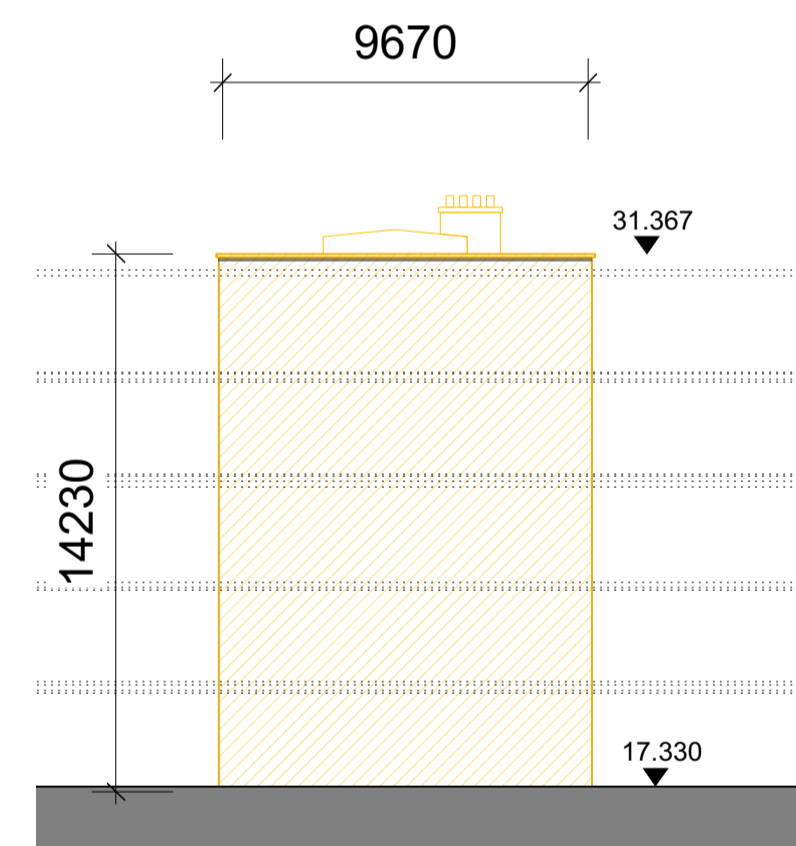
3 Existing And Demolition South Elevation 030204 1:200 @ A1
