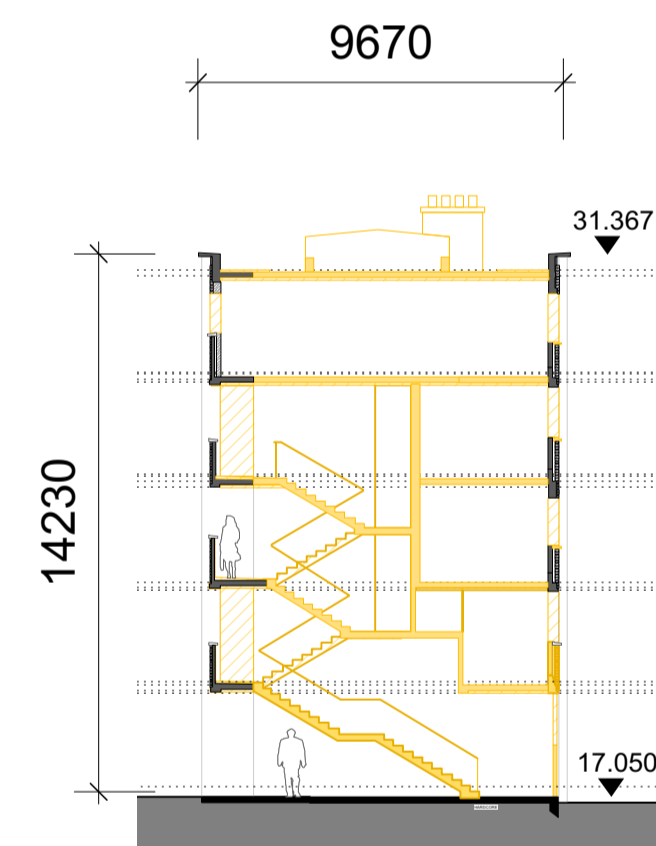
5 Existing And Demolition Core Section 030204 1:200 @ A1
