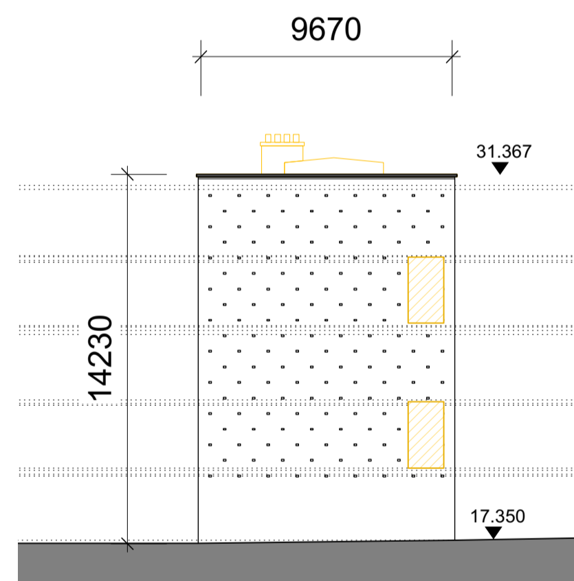
6 Existing And Demolition North Elevation 030204 1:200 @ A1
