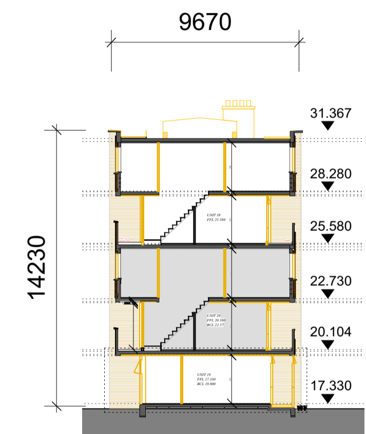
6 Existing And Demolition Typical Section 030204 1:200 @ A1
