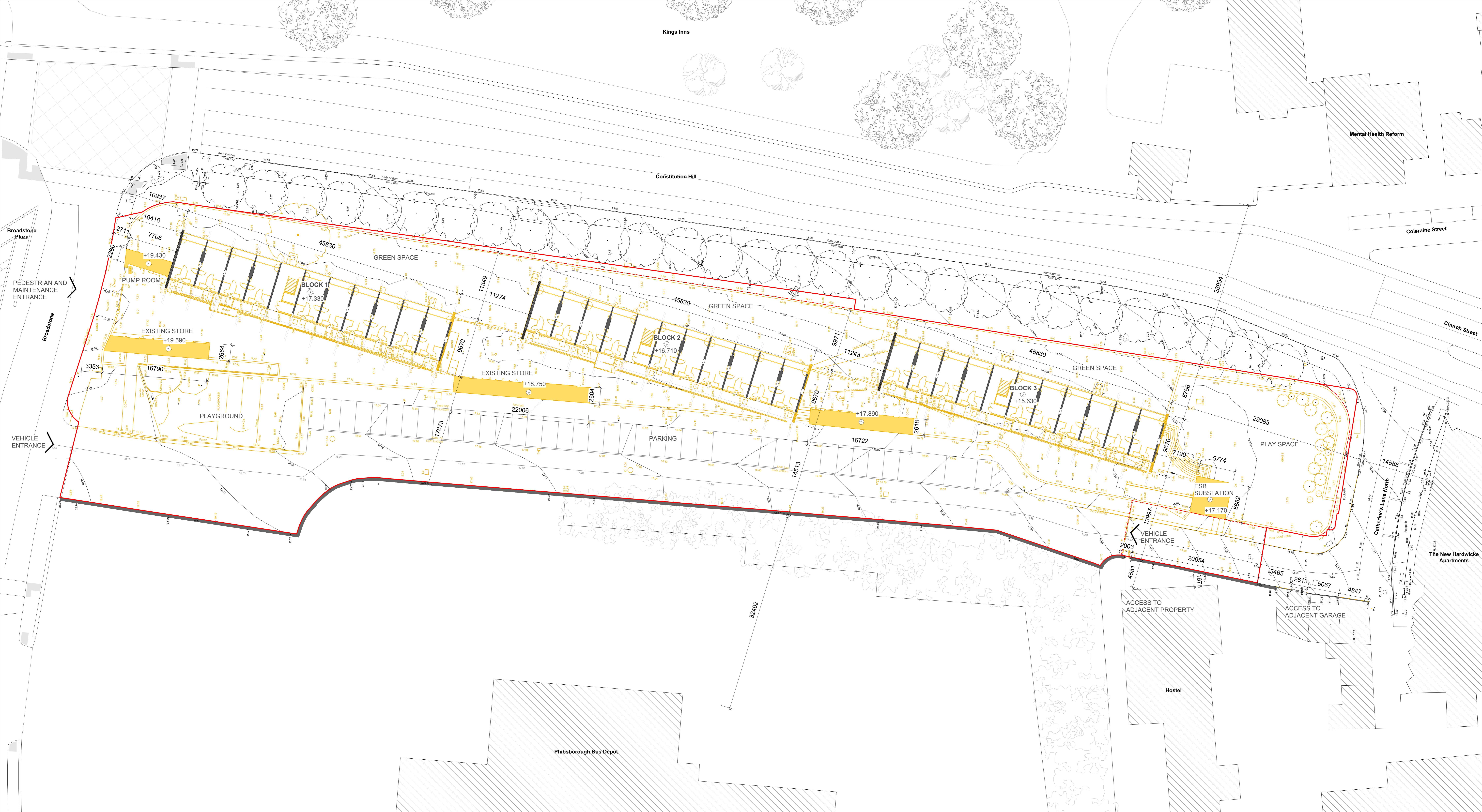
1 Existing General Arrangement Site Plan L00 - with demolition 1:200 @ A0
